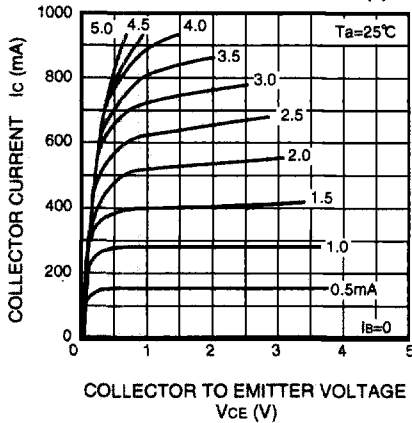
COMMON EMITTER OUTPUT (1)
