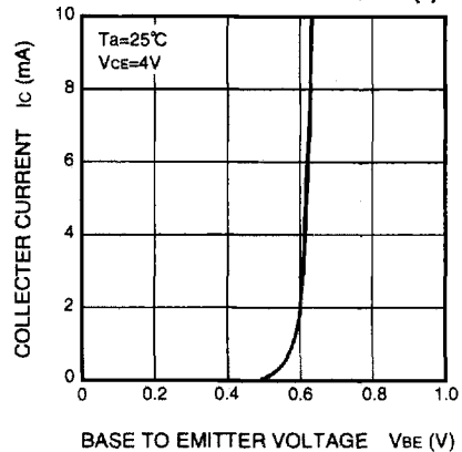
COMMON EMITTER TRANSFER (2)
