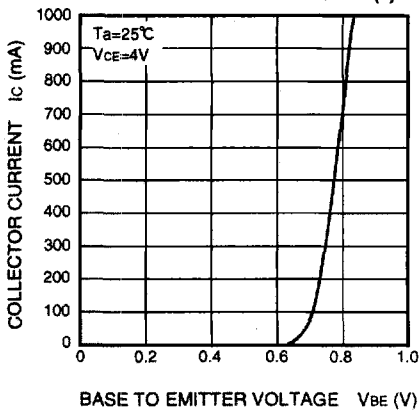
COMMON EMITTER TRANSFER (1)
