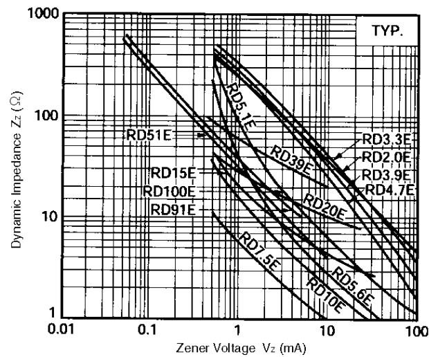
Figure 4. Z_z vs. I_z Example of Characteristics
