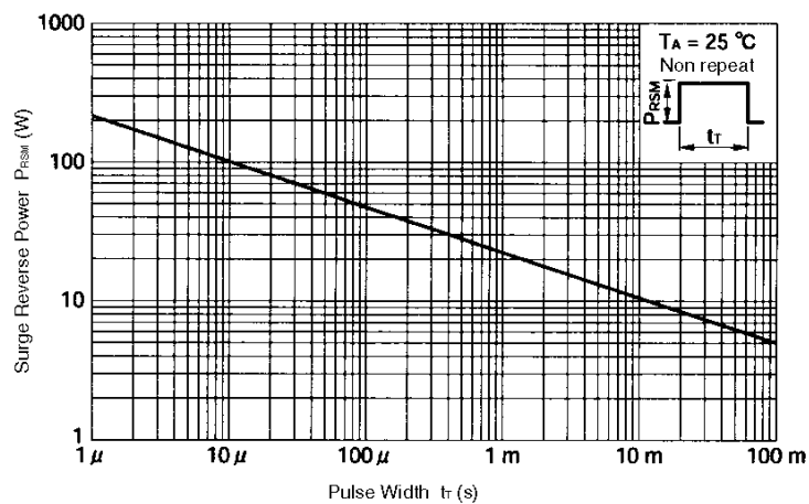
Figure 6. Surge Reverse Power Rating
