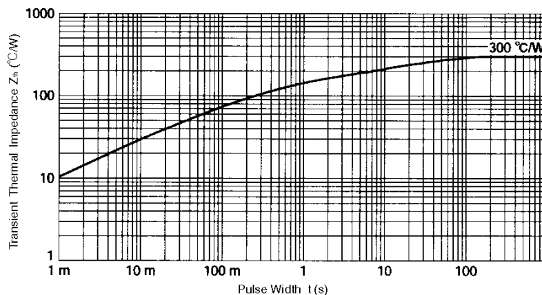
Figure 7. Transient Heat Thermal Impedance
