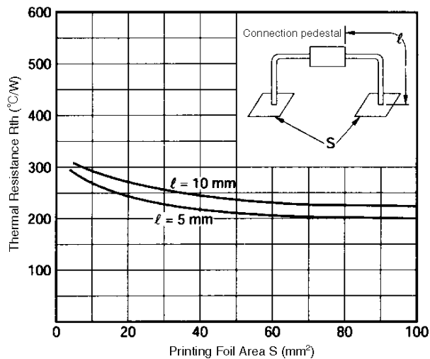
Figure 2. S vs. R_{th} Example of Characteristics
