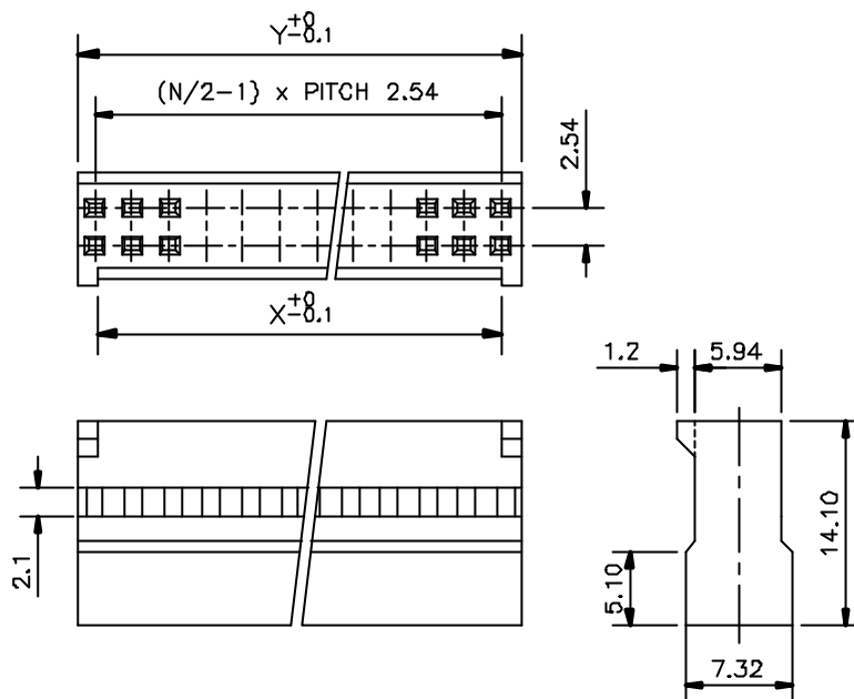
FEMALE CRIMP INSULATOR
