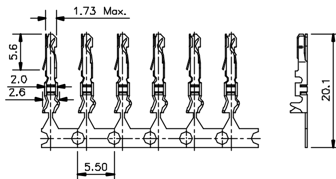
FEMALE CRIMP CONTACT
