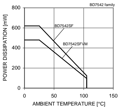
Fig. 71 Derating Curve
