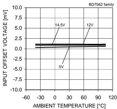
Fig. 37 Input Offset Voltage – Ambient Temperature (Vicm=VDD, VOUT=VDD/2)
