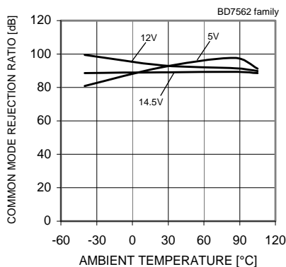
Fig. 42 Common Mode Rejection Ratio – Ambient Temperature (VDD=12[V])
