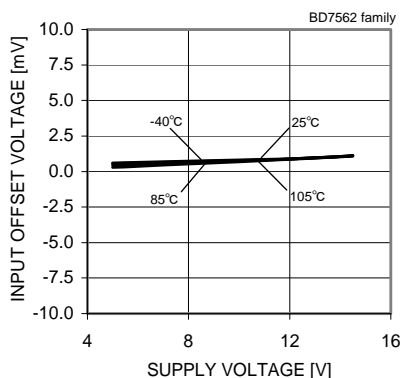
Fig. 36 Input Offset Voltage – Supply Voltage (Vicm=VDD, VOUT=VDD/2)
