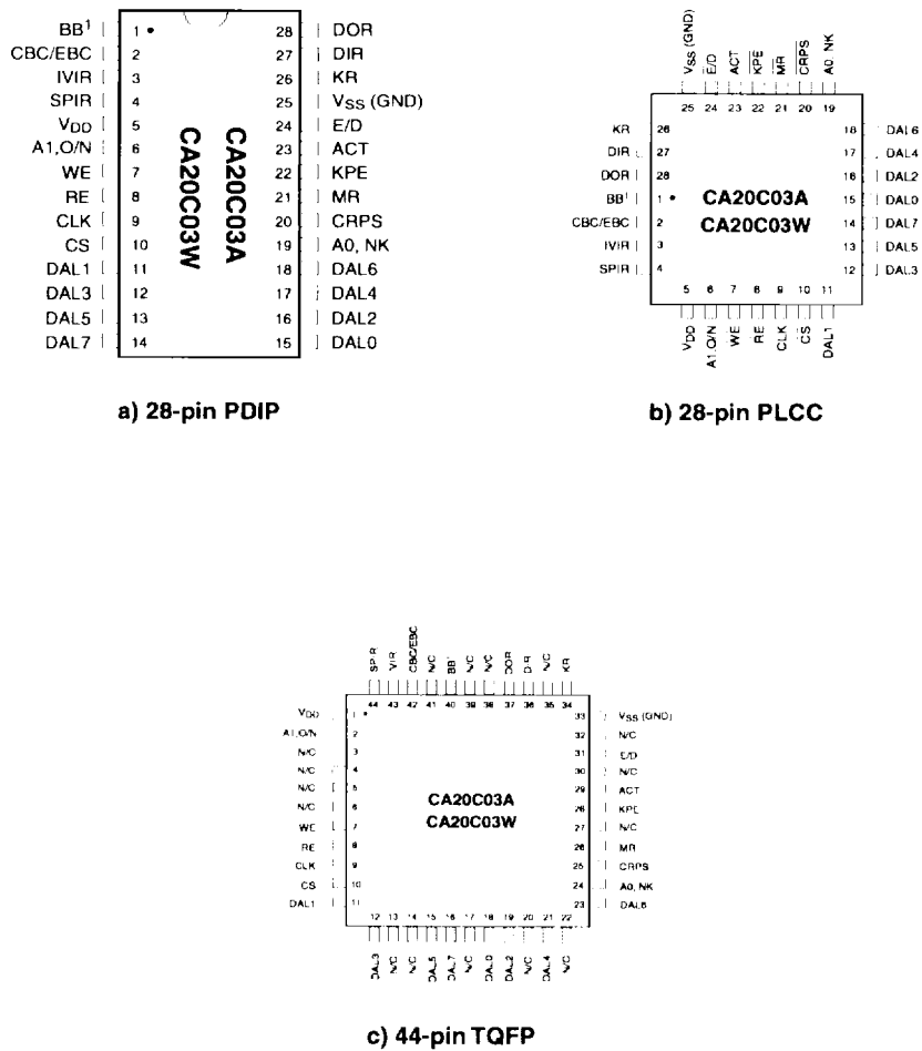
Figure 3-2 : CA20C03A/W Pin Configurations
