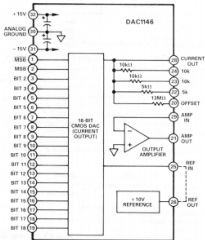
Figure 1. DAC1146 Block Diagram
