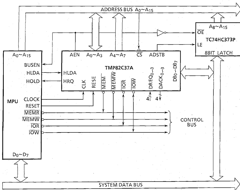
Figure 11.1 Basic System Connection Diagram
