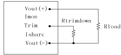
Figure 17: Circuit configuration for trim-down (decrease output voltage)
