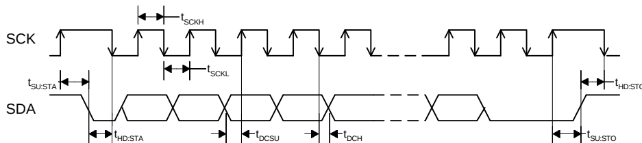
Figure 7. Data Interface Timing (I²C)
