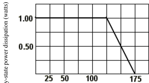
T_L – lead Temperature FIG. 3 Steady-state power derating curve
