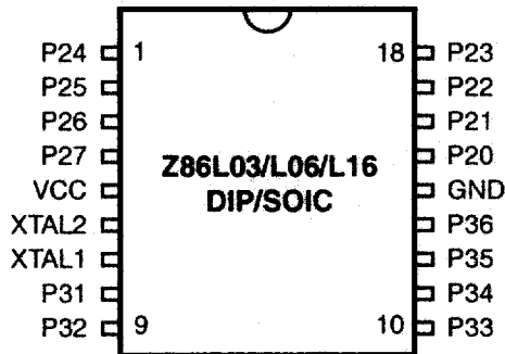
Figure 2. 18-Pin DIP/SOIC Configuration
