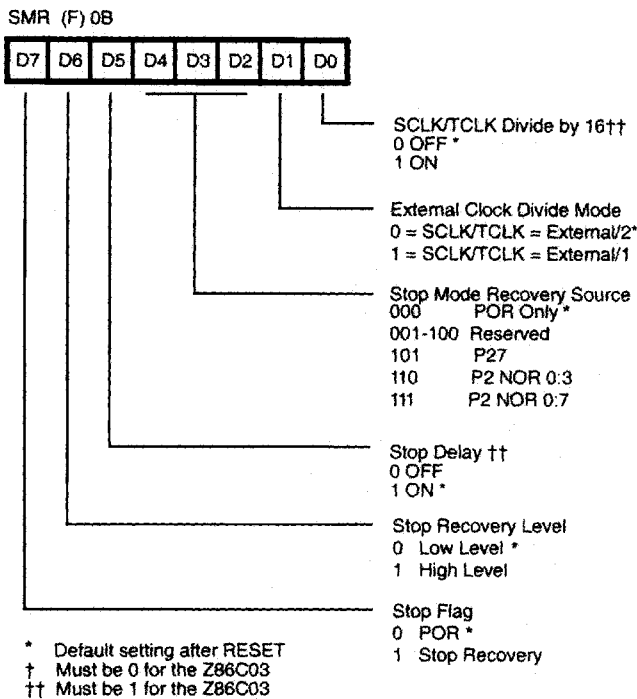
Figure 16. Stop-Mode Recovery Register (Write Only except bit D7, which is Read Only.) (Z86L06/16)
