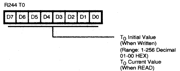
Figure 29. Counter/Timer 0 Register (F4H: Read/Write; Z86L06 Only)
