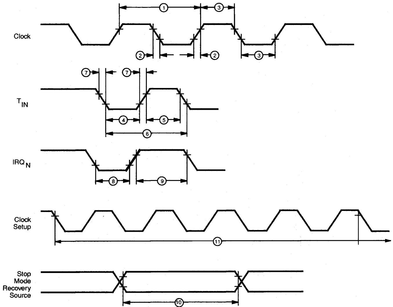
Figure 4. Additional Timing
