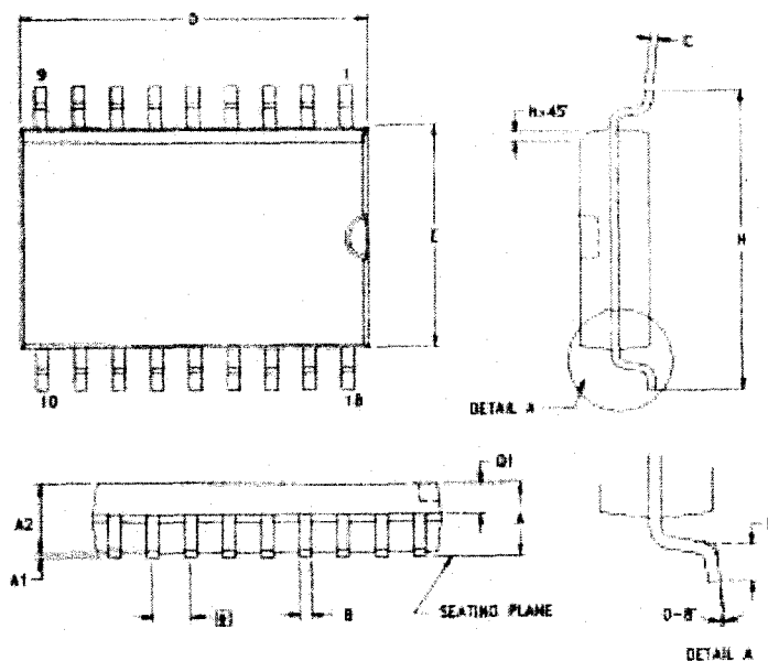
Figure 42. 18-Pin SOIC Package Diagram
