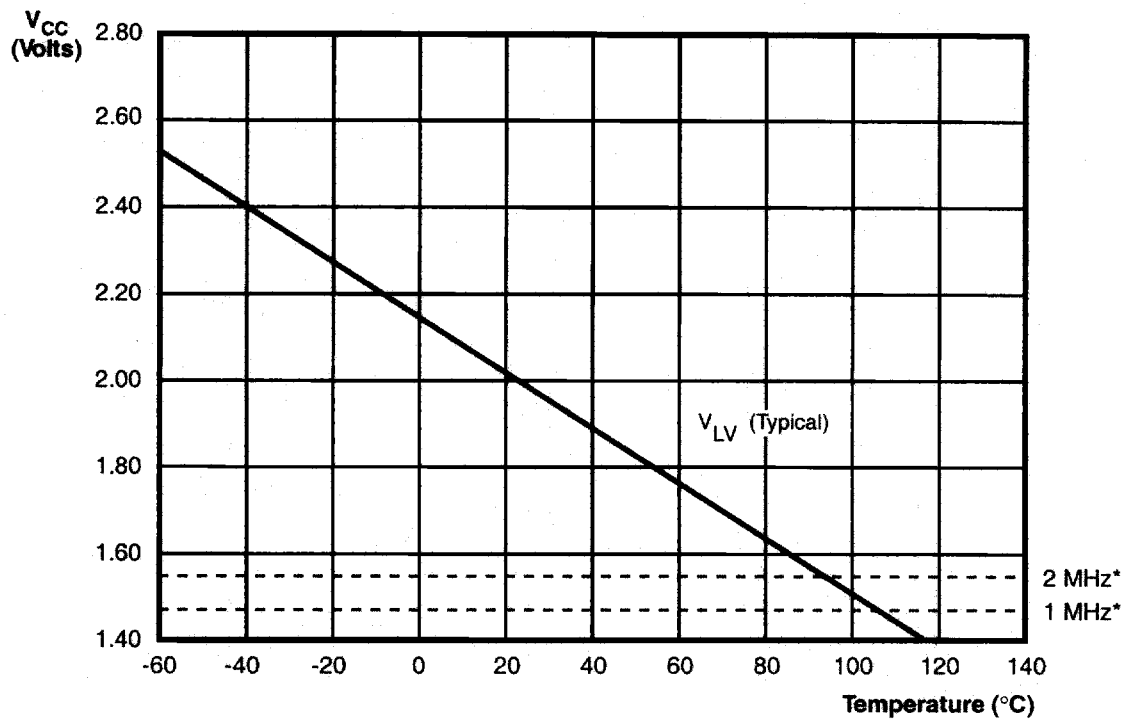
Figure 21. Typical Z86L03/L06/L16 V_{LV} Voltage vs Temperature
