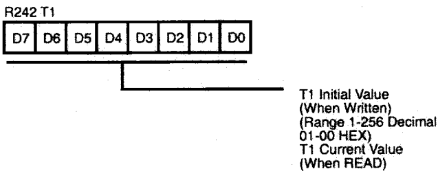
Figure 27. Counter Timer 1 Register (F2H: Read/Write)
