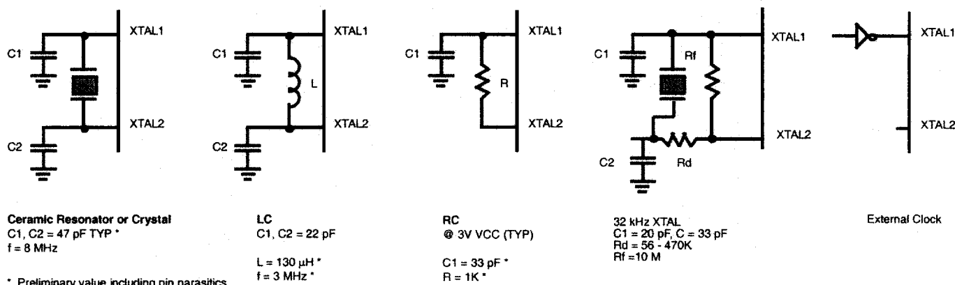
Figure 13. Oscillator Configuration
