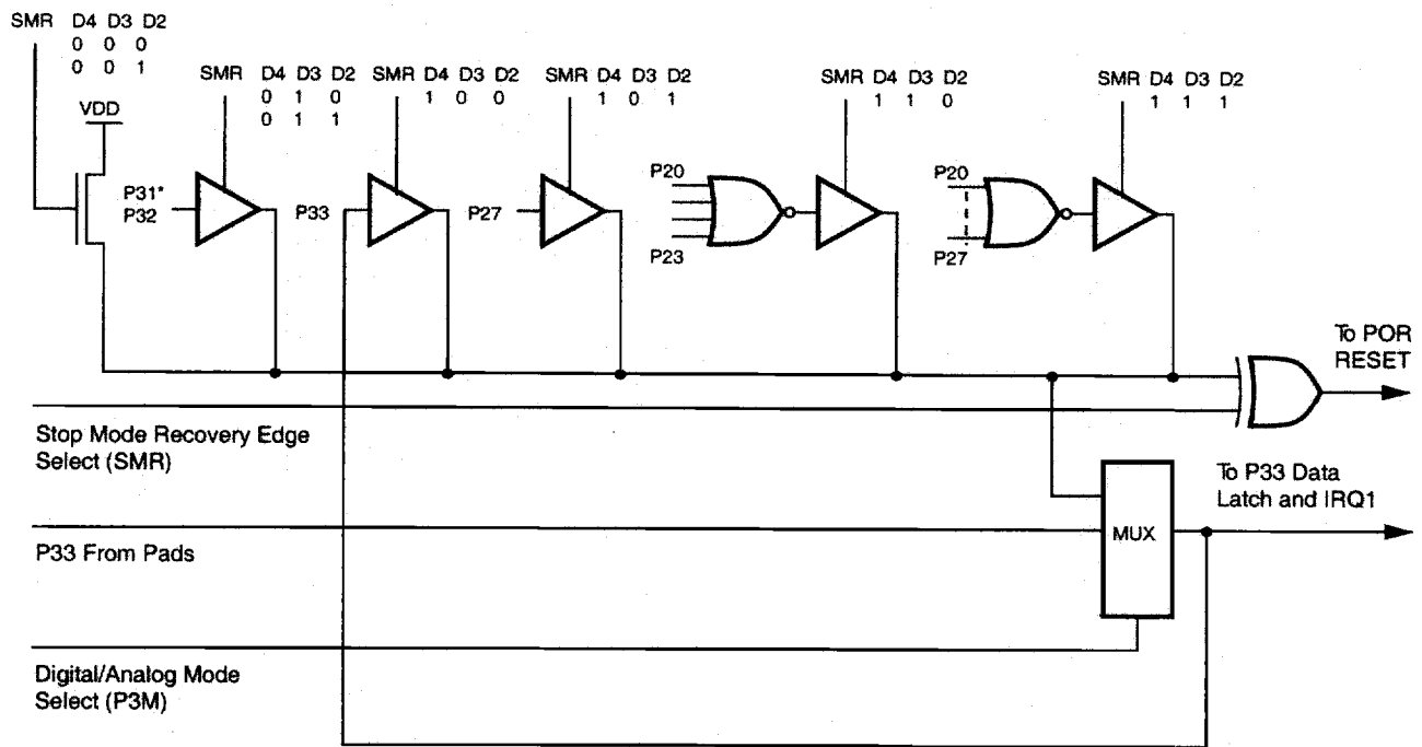
Figure 18. Stop-Mode Recovery Source (Z86L06/16)
