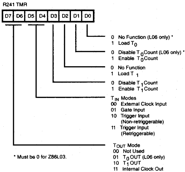
Figure 26. Timer Mode Register (F1H: Read/Write)
