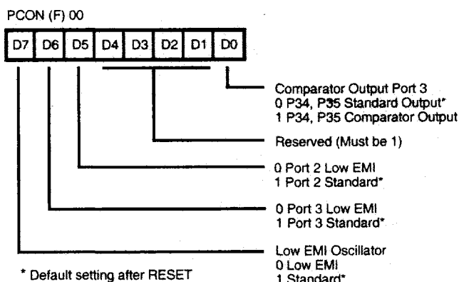
Figure 14. Port Configuration Register (PCON) (Write Only)
