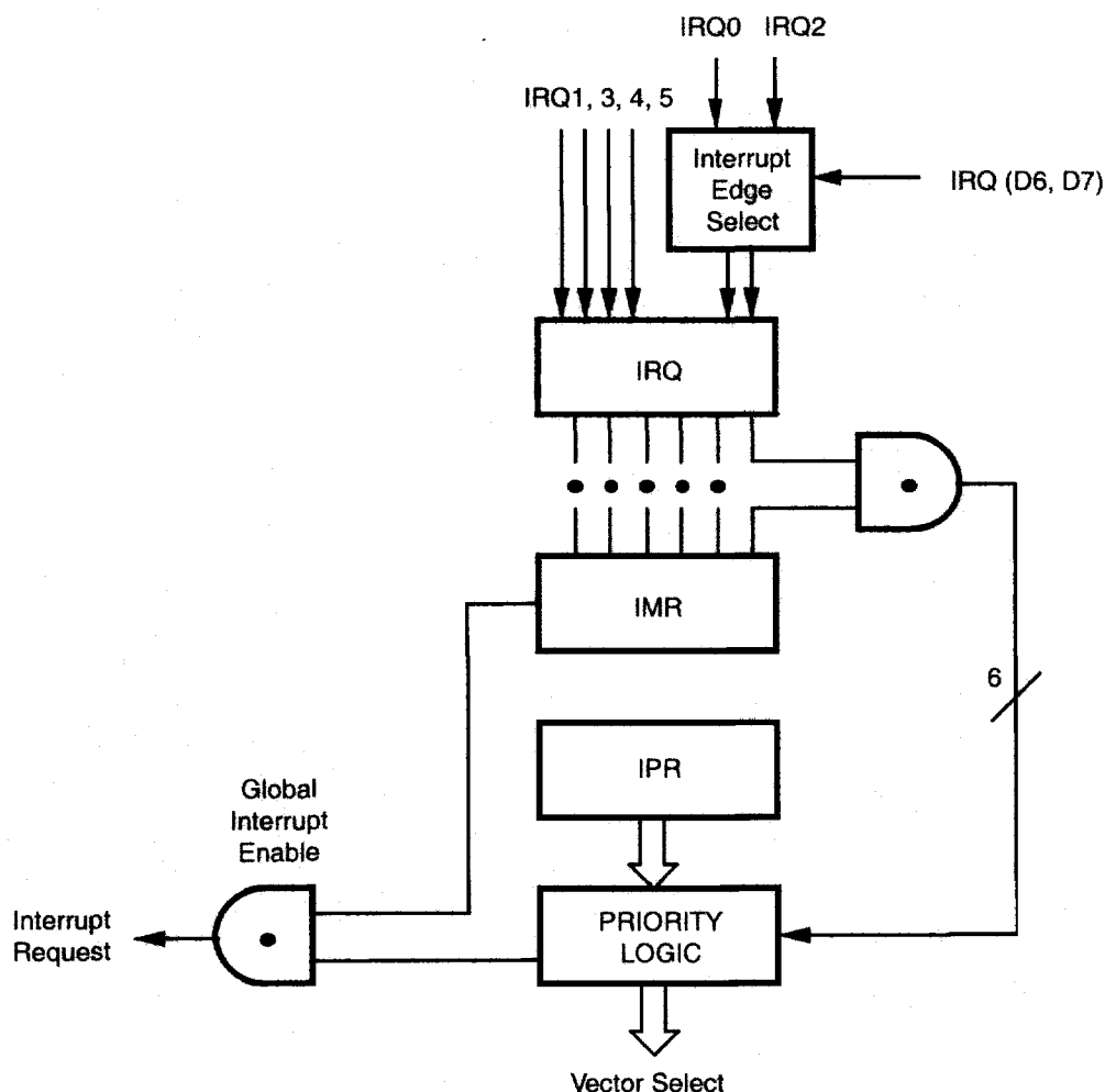
Figure 12. Interrupt Block Diagram
