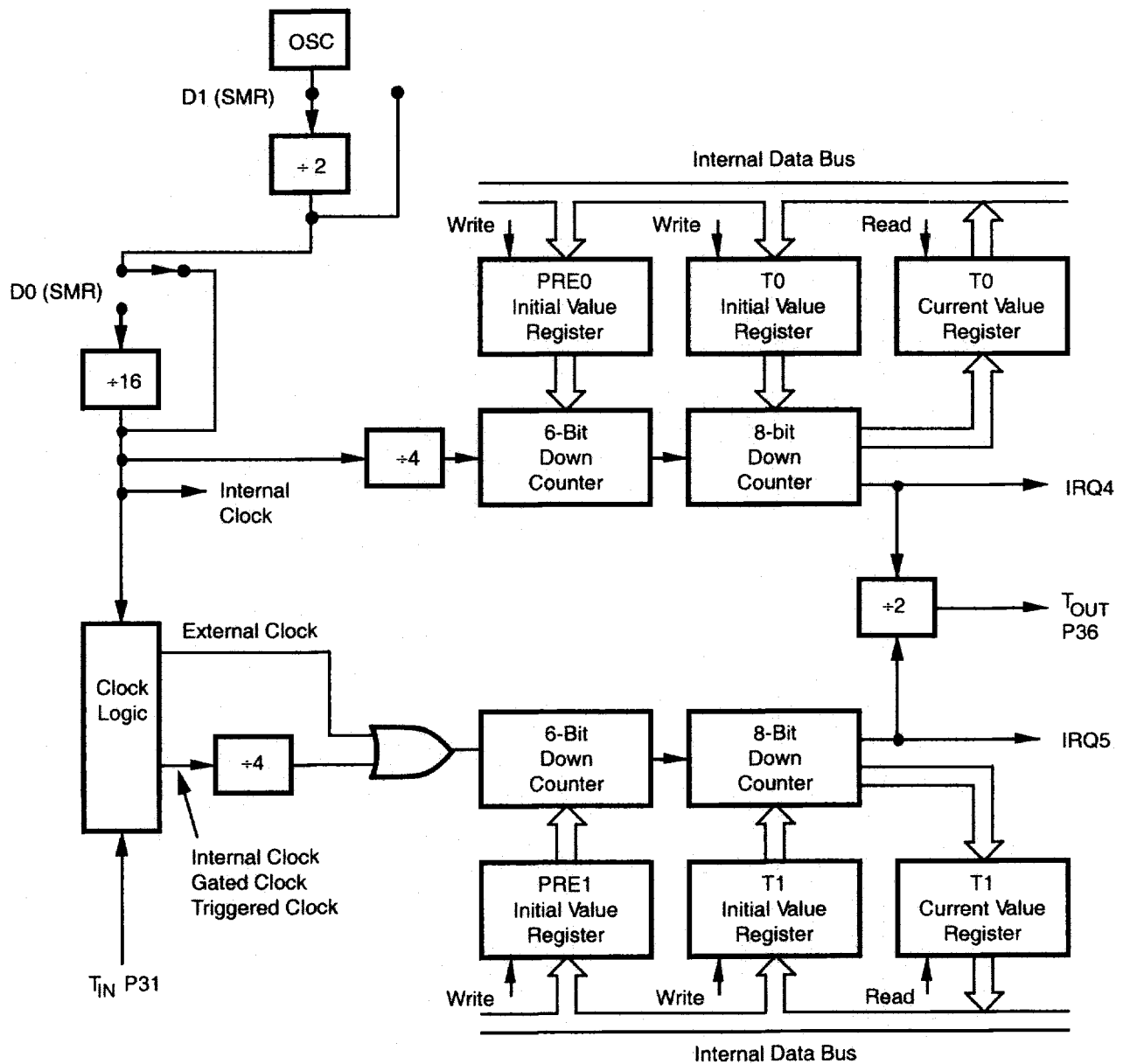
Figure 11. Counter/Timer Block Diagram
