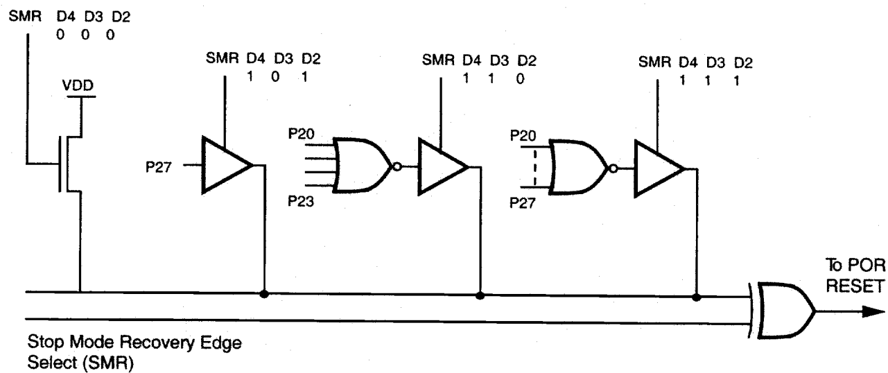
Figure 17. STOP-Mode Recovery Source (Z86L03)
