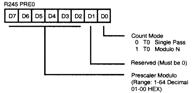
Figure 28. Prescaler 1 Register (F3H: Write Only)
