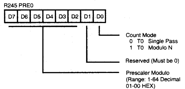
Figure 30. Prescaler 0 Register (F5H: Write Only; Z86L06 Only)
