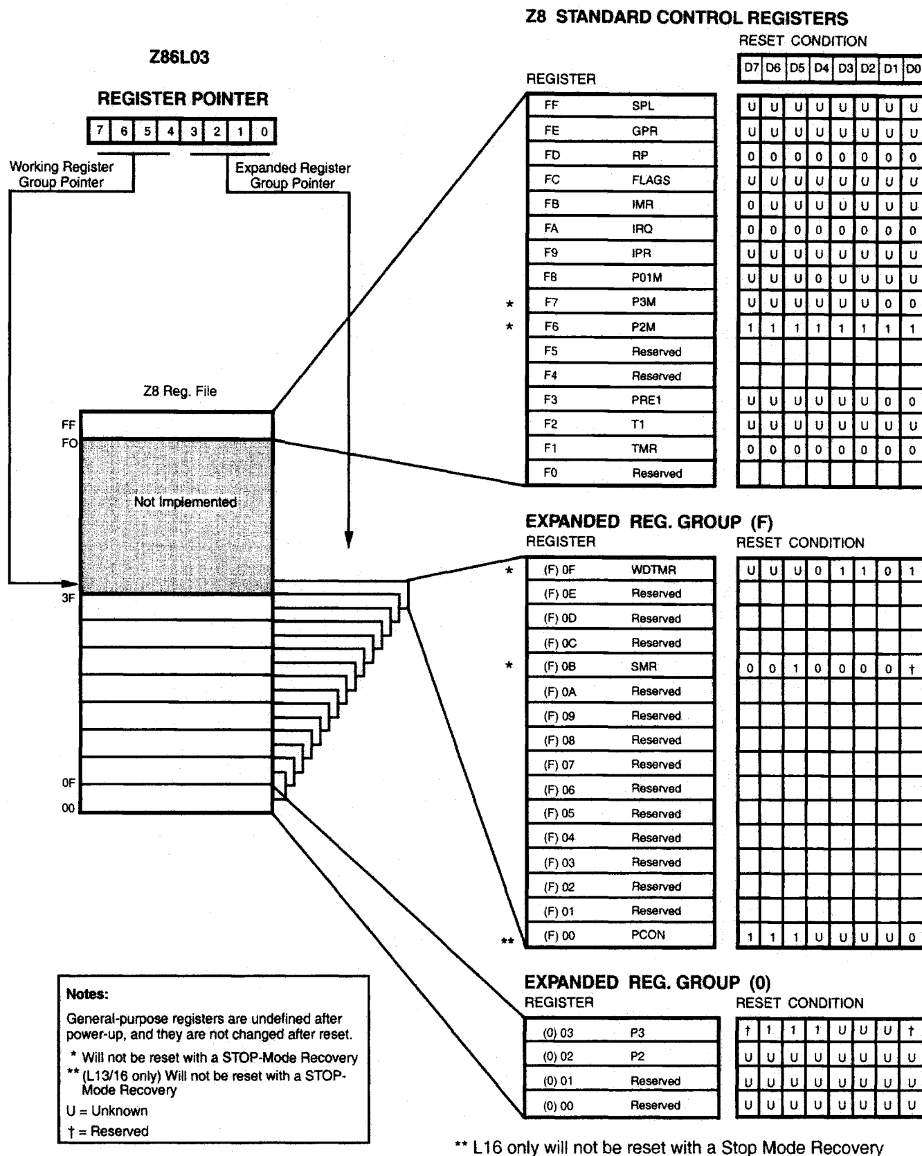
Figure 8. Expanded Register File Architecture
