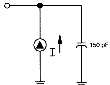
Figure 3. Test Load Configuration
