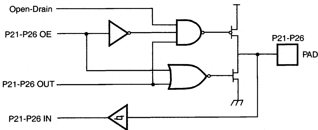
Figure 5. Port 2 Configuration
