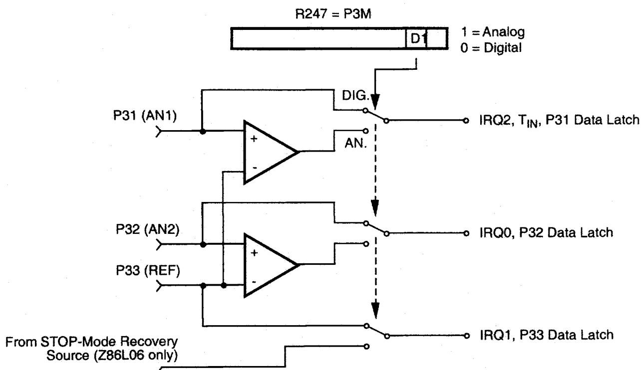
Figure 6. Port 3 Configuration
