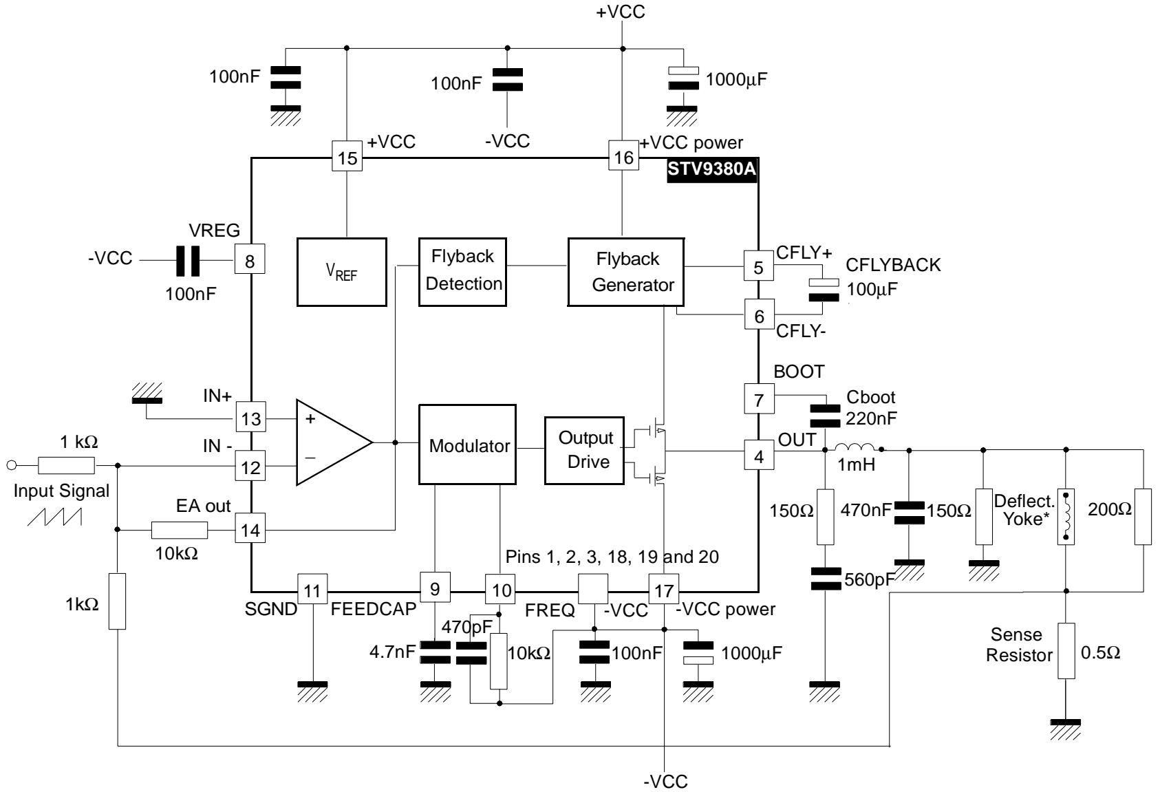
Figure 1 : Test and Application Circuit Diagram
