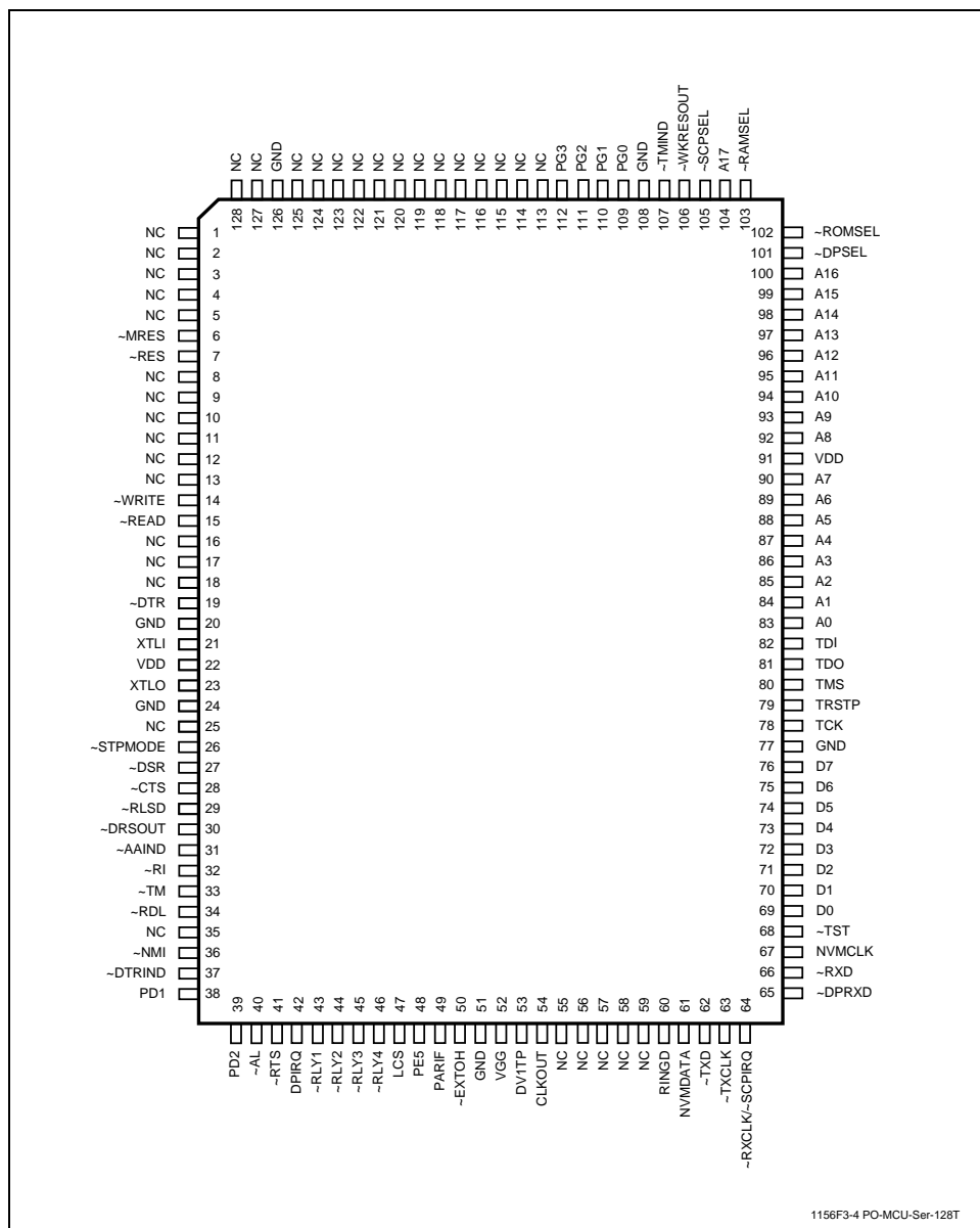
Figure 9. MCU Pin Signals - Serial DTE Interface - 128-Pin TQFP
