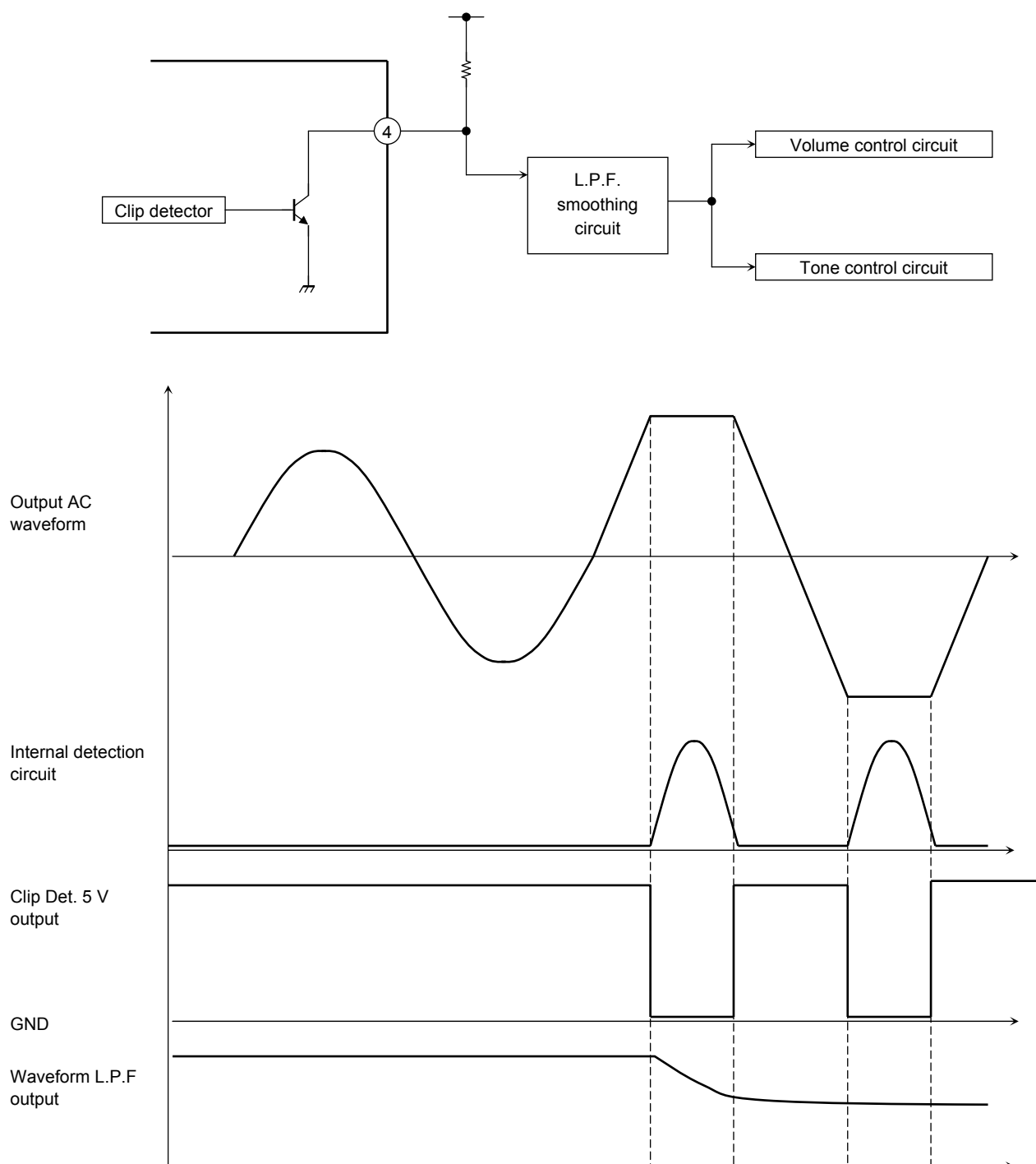
Figure 1 Clip Detection
