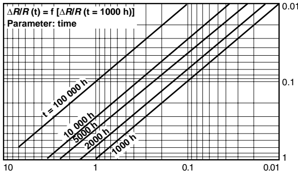
Stability nomogram typical values (for handling see general explanations)
