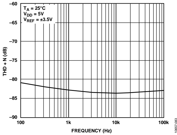
Figure 23. THD + Noise vs. Frequency
