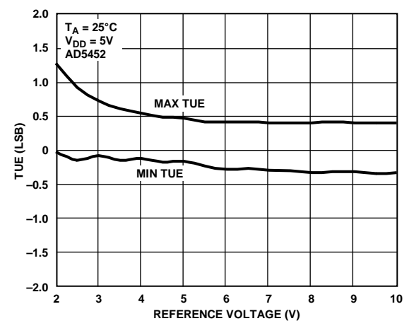
Figure 9. TUE vs. Reference Voltage
