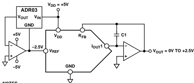
Figure 36. Positive Output Voltage with Minimum Components
