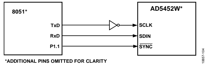
Figure 44. 80C51/80L51-to-AD5452W Interface
