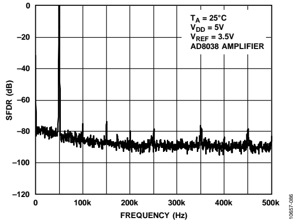
Figure 26. Wideband SFDR, f_{OUT} = 50 kHz, Clock = 1 MHz
