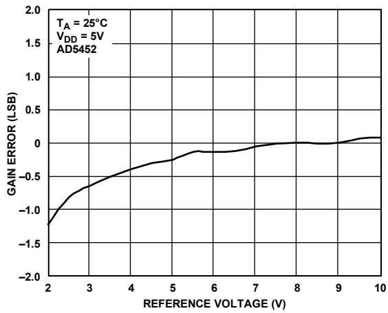
Figure 11. Gain Error (LSB) vs. Reference Voltage
