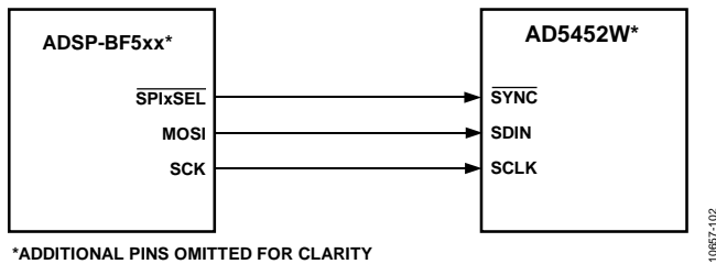
Figure 42. ADSP-BF5xx-to-AD5452W Interface
