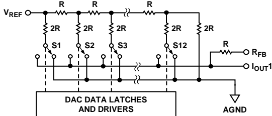
Figure 32. AD5452W Simplified Ladder
