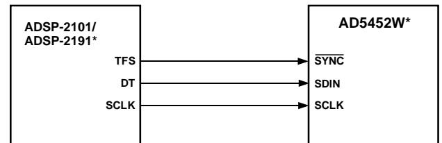
Figure 41. ADSP-2101/ADSP-2191 PORT-to-AD5452W Interface
