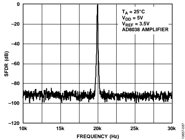
Figure 27. Narrow-Band SFDR, f_{OUT} = 20 kHz, Clock = 1 MHz
