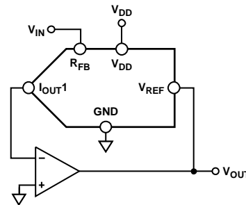
Figure 38. Current-Steering DAC Used as a Divider or Programmable Gain Element
