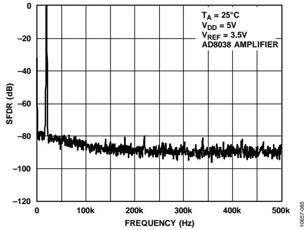
Figure 25. Wideband SFDR, f_{OUT} = 20 kHz, Clock = 1 MHz
