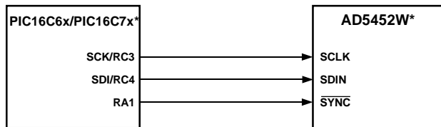
Figure 47. PIC16C6x/7x-to-AD5452W Interface
