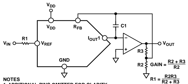
Figure 37. Increasing Gain of Current-Output DAC
