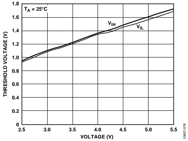
Figure 16. Threshold Voltage vs. Supply Voltage
