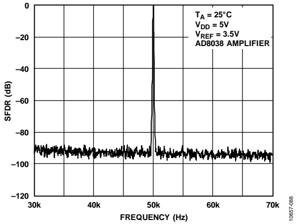
Figure 28. Narrow-Band SFDR, f_{OUT} = 50\text{ kHz} , Clock = 1 MHz
