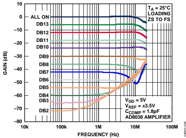
Figure 17. Reference Multiplying Bandwidth vs. Frequency and Code
