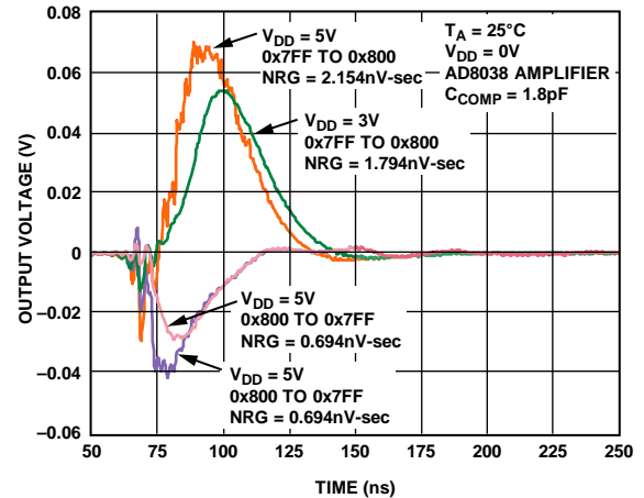
Figure 20. Midscale Transition, V_{REF} = 0\text{ V}
