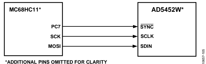
Figure 45. MC68HC11-to-AD5452W Interface
