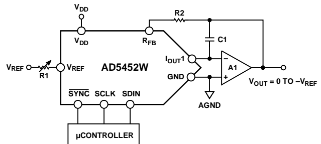
Figure 33. Unipolar Mode Operation
