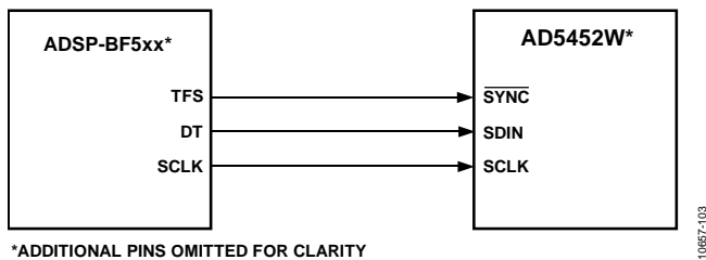
Figure 43. ADSP-BF5xx SPORT-to-AD5452W Interface
