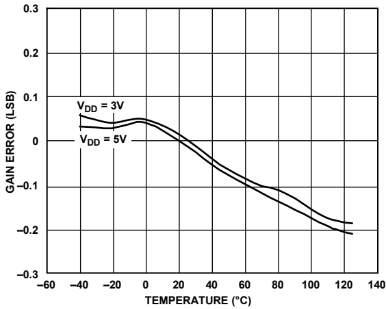
Figure 10. Gain Error (LSB) vs. Temperature
