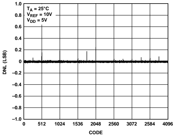
Figure 5. DNL vs. Code
