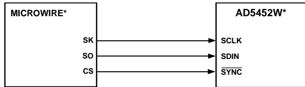
Figure 46. MICROWIRE-to-AD5452W Interface
