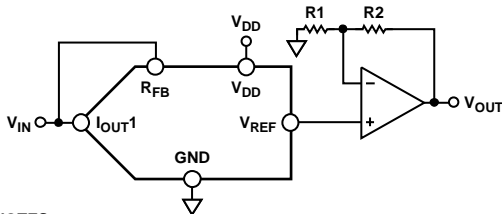
Figure 35. Single-Supply Voltage-Switching Mode
