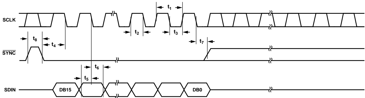
Figure 2. Timing Diagram
