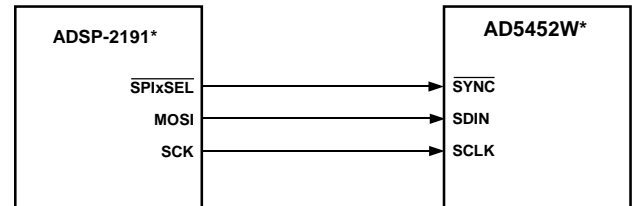
Figure 40. ADSP-2191 SPI-to-AD5452W Interface
