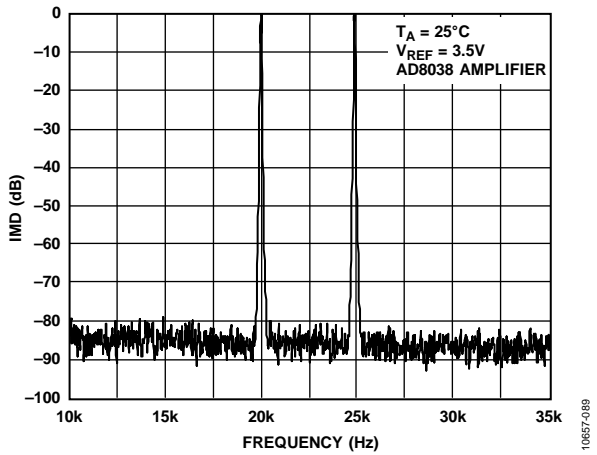
Figure 29. Narrow-Band IMD, f_{OUT} = 20\text{ kHz}, 25\text{ kHz} , Clock = 1 MHz
