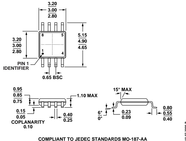
COMPLIANT TO JEDEC STANDARDS MO-187-AA Figure 48. 8-Lead Mini Small Outline Package [MSOP] (RM-8) Dimensions shown in millimeters
