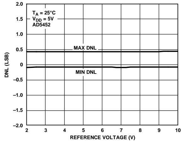
Figure 7. DNL vs. Reference Voltage
