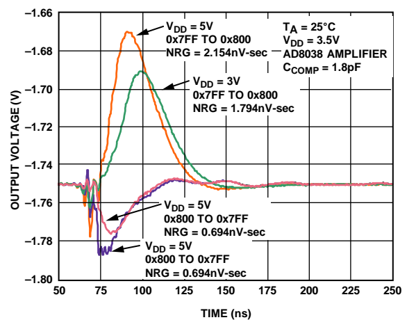
Figure 21. Midscale Transition, V_{REF} = 3.5\text{ V}
