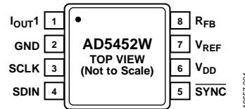
Figure 3. Pin Configuration
