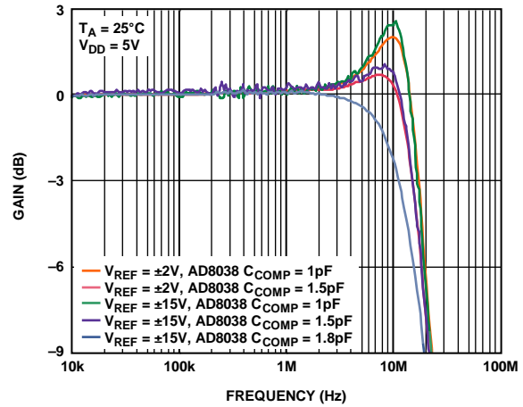
Figure 19. Reference Multiplying Bandwidth vs. Frequency and Compensation Capacitor
