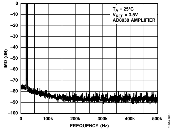
Figure 30. Wideband IMD, f_{OUT} = 20\text{ kHz}, 25\text{ kHz} , Clock = 1 MHz
