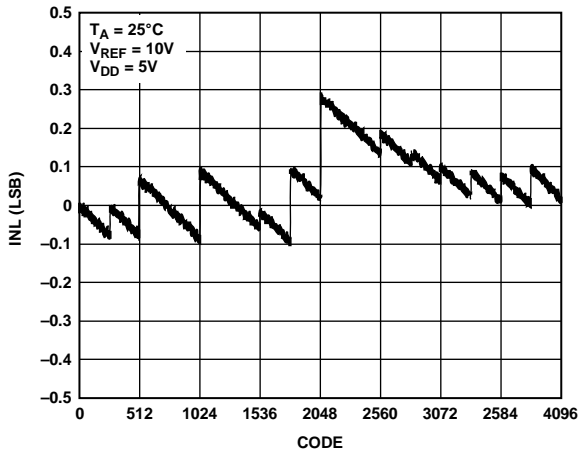
Figure 4. INL vs. Code
