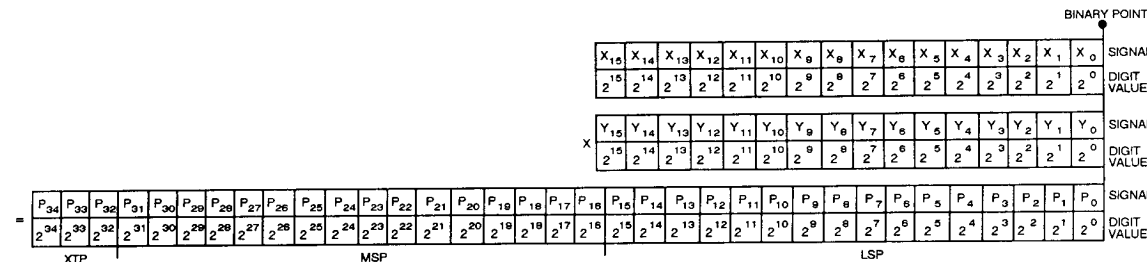
Figure 9. Integer Unsigned Magnitude Notation
