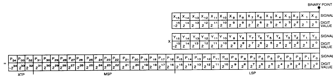
Figure 8. Integer Two's Complement Notation
