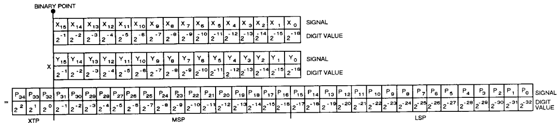
Figure 7. Fractional Unsigned Magnitude Notation
