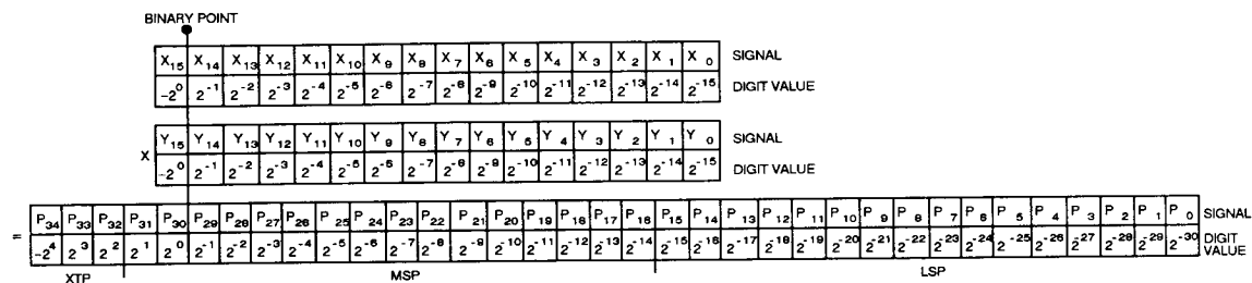
Figure 6. Fractional Two's Complement Notation
