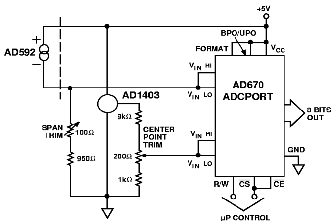
Figure 13. Temperature to Digital Output
