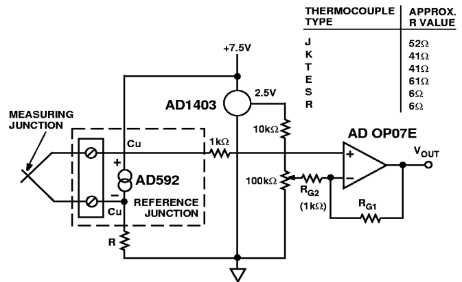
Figure 11. Thermocouple Cold Junction Compensation
