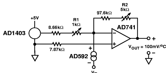
Figure 6. Two Temperature Trim Circuit
