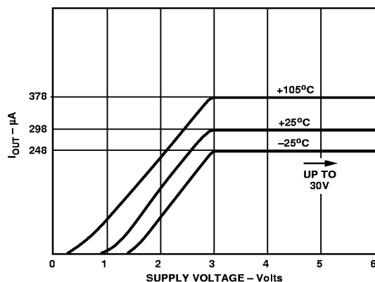
Figure 1. V-I Characteristics
