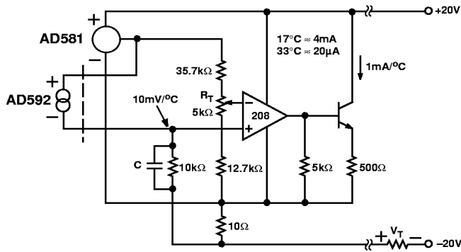
Figure 12. Temperature to 4–20 mA Current Transmitter
