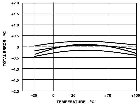
AD592CN Accuracy Over Temperature
