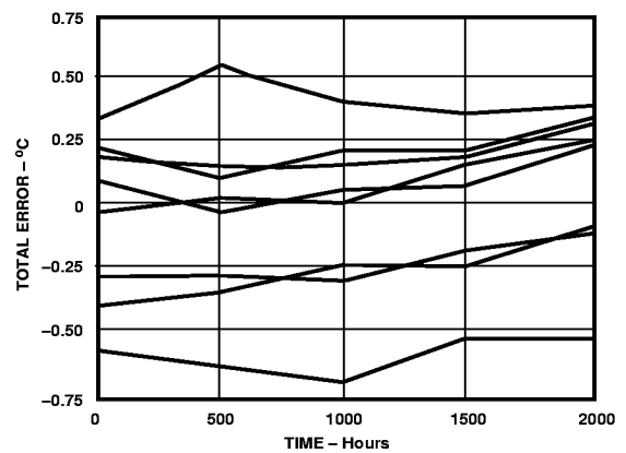
Long-Term Stability @ +85°C and 85% Relative Humidity
