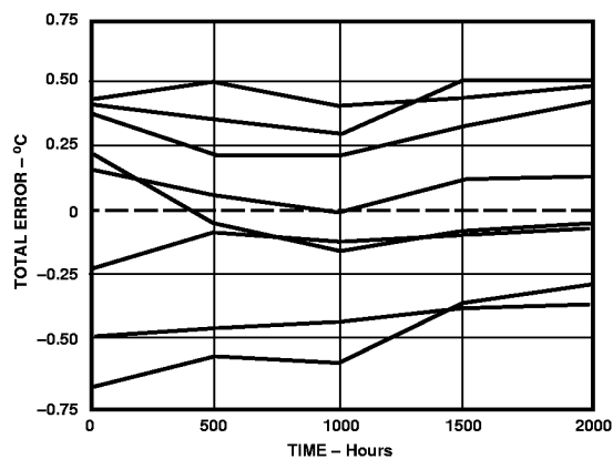
Long-Term Stability @ +125°C
