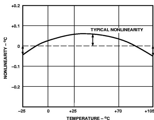
Figure 3. Nonlinearity Error (AD592CN)
