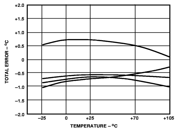
AD592BN Accuracy Over Temperature
