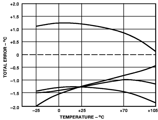
AD592AN Accuracy Over Temperature
