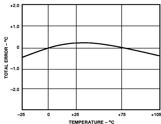
Figure 7. Typical Two Trim Accuracy
