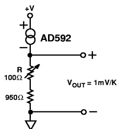
Figure 4. Basic Voltage Output (Single Temperature Trim)
