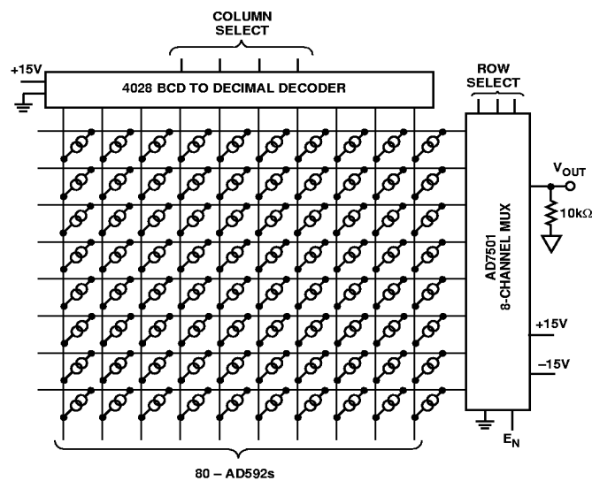
Figure 16. Matrix Multiplexer
