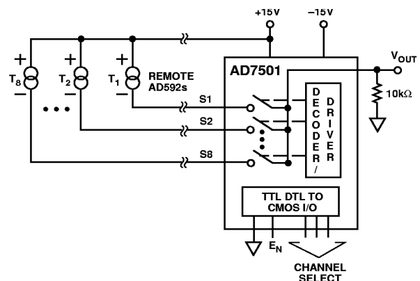
Figure 15. Remote Temperature Multiplexing
