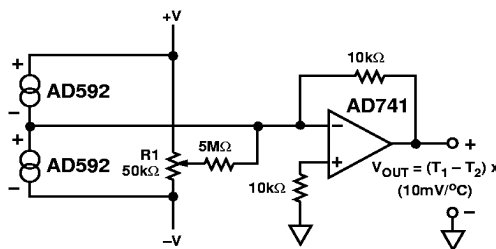
Figure 10. Differential Measurements
