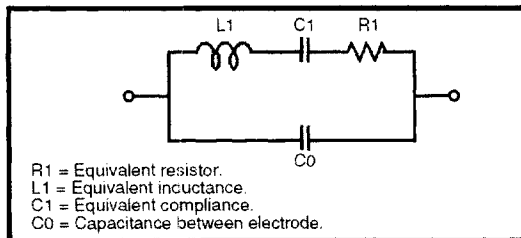
Resonator and Crystal Electric Equivalent Circuit
