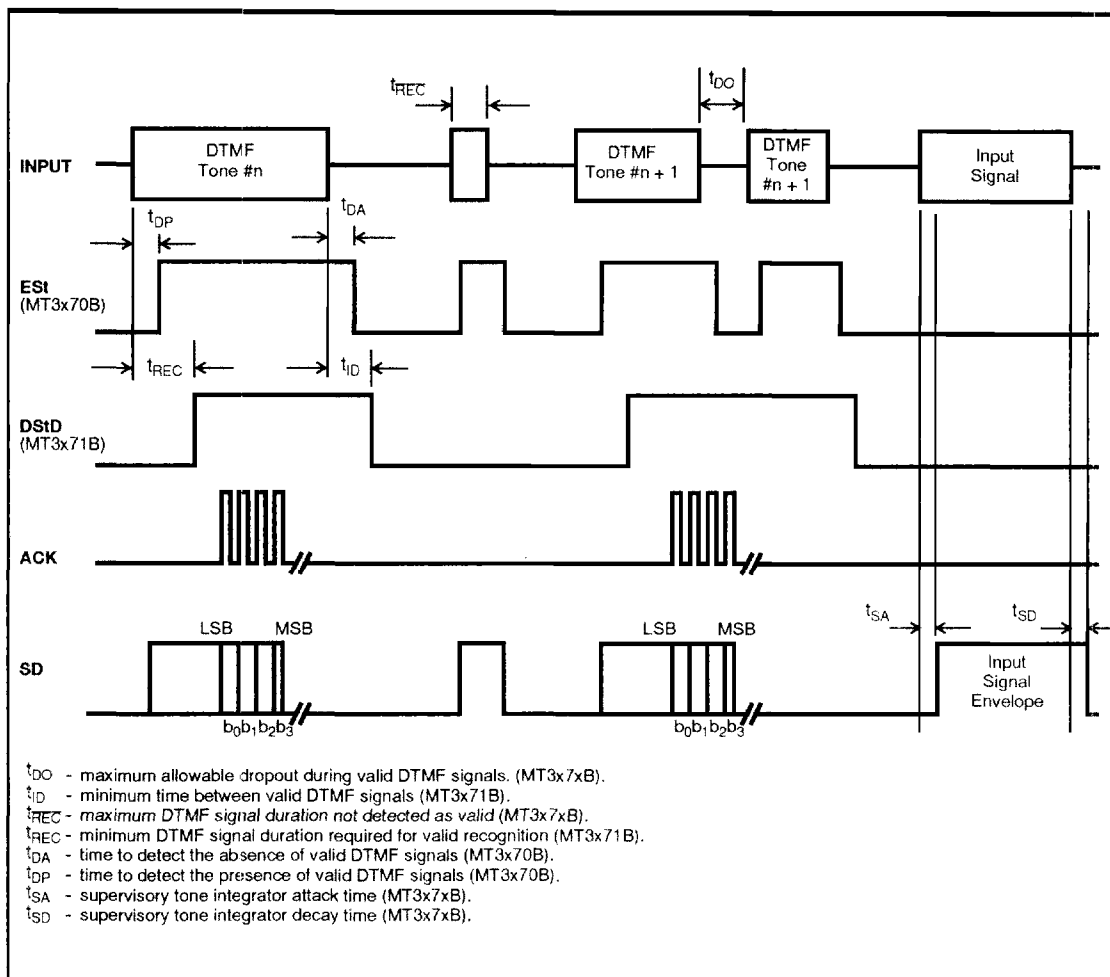
Figure 4 - Timing Diagram
