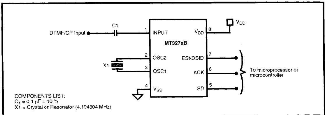
Figure 3 - Application Circuit for MT327xB
