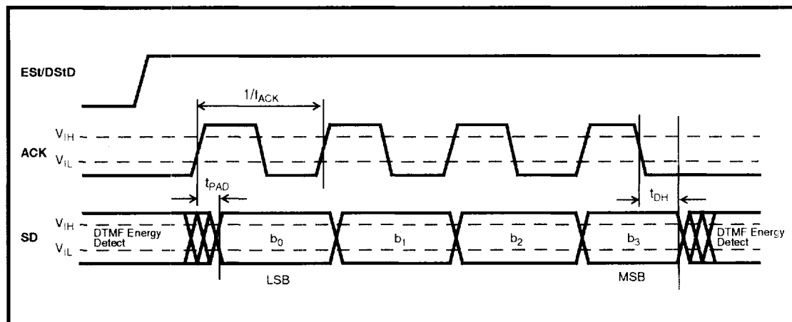
Figure 5 - ACK to SD Timing
