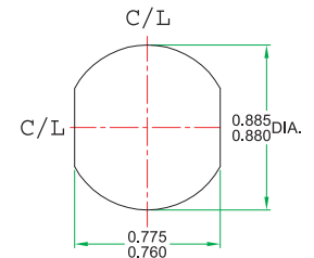
SUGGESTED MOUNTING HOLE
