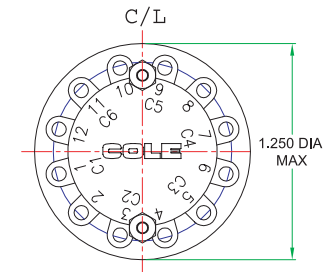
60° INDEXING
