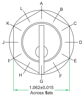
30° INDEXING
