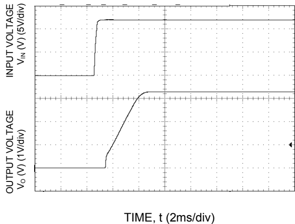
Figure 26. Typical Start-up Using Input Voltage (VIN = 12V, I o = I o,max ).
