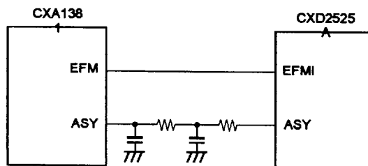
Application Circuit
