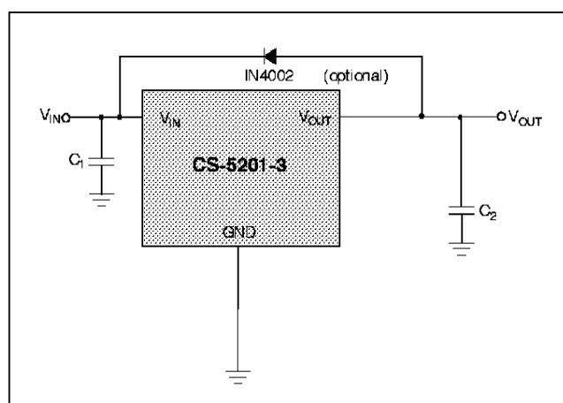
Figure 1. Protection diode scheme for large output capacitors.
