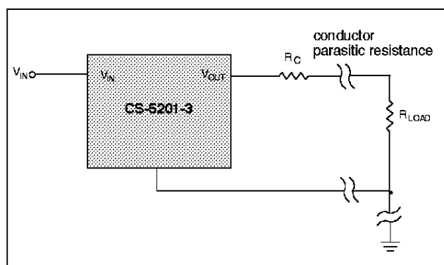
Figure 2. Conductor parasitic resistance effects can be minimized with the above grounding scheme for fixed output regulators.
