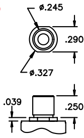
NON-THREADED
