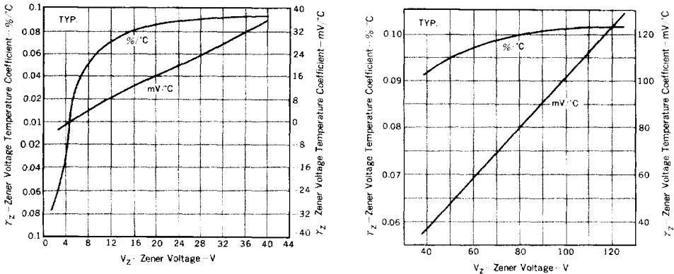
Fig. 3 \gamma_Z - V_Z CHARACTERISTICS
