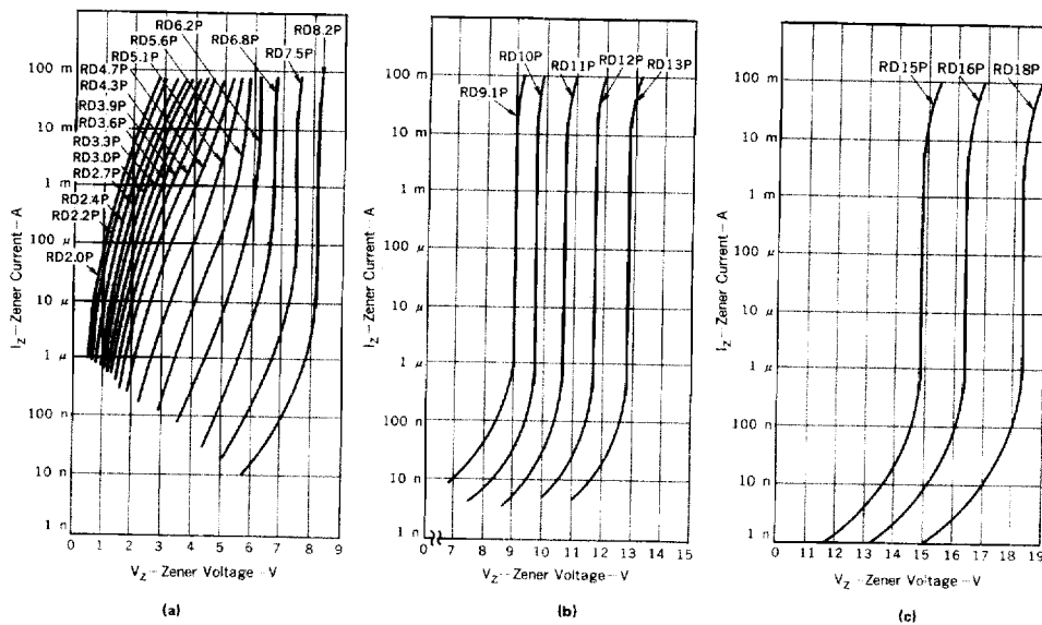
Fig. 2 i_z - v_z CHARACTERISTICS
