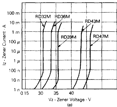
Fig. 3 V_z - V_z CHARACTERISTICS
