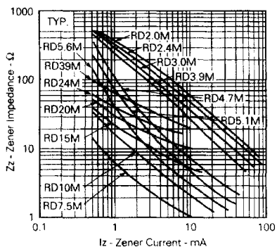
Fig. 4 Z_z - I_z CHARACTERISTICS
