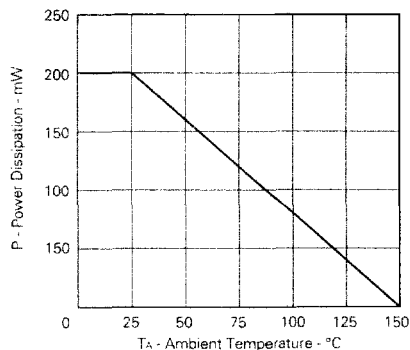
Fig. 1 P- T_A RATING
