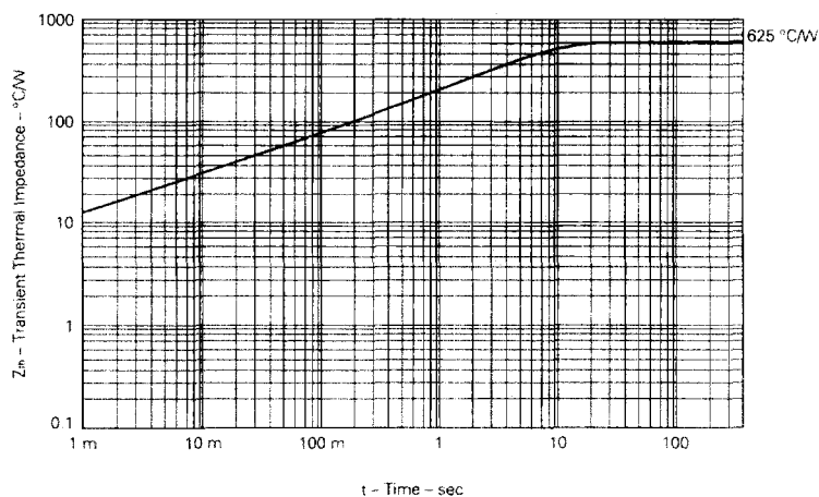
Fig. 5 TRANSIENT THERMAL IMPEDANCE CHARACTERISTICS
