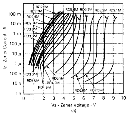
Fig. 2 I_Z - V_Z CHARACTERISTICS (a to e)
