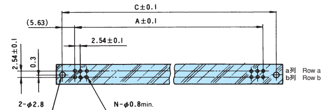
推奨取付寸法 Recommended mounting dimensions
