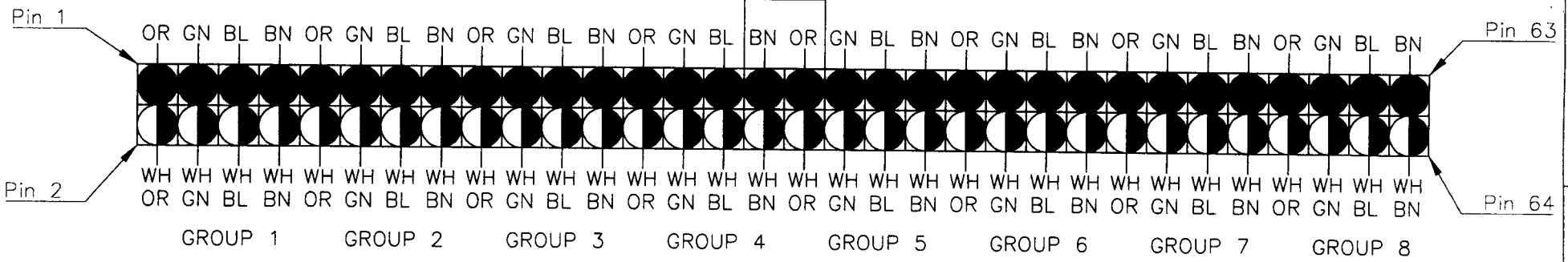
UPPER VERSION VIEWED FROM REAR.
