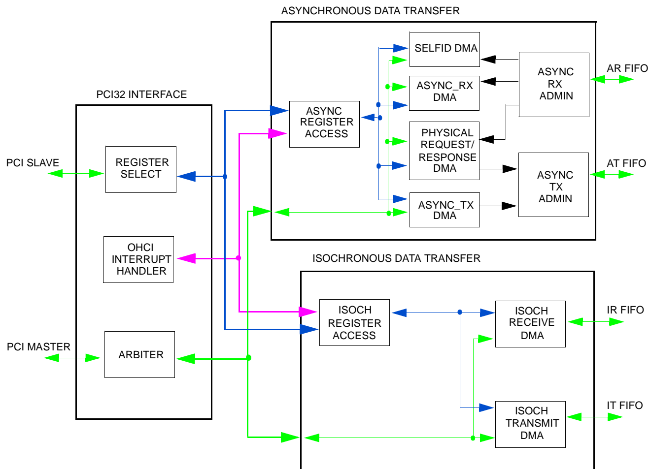
Figure 3. OHCI Core Block Diagram
