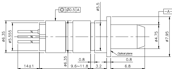
SC TOSA C-XXXXX-DFB2.5-TX-SSCXX
