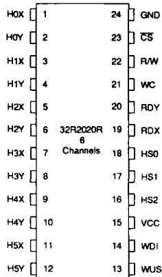
24-Pin SOV
