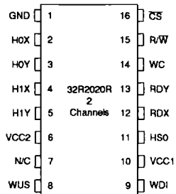
16-Pin SOL
