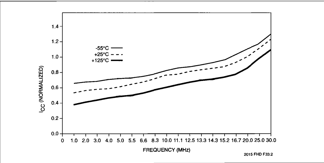
Normalized I_{CC} by Temperature over Frequency
