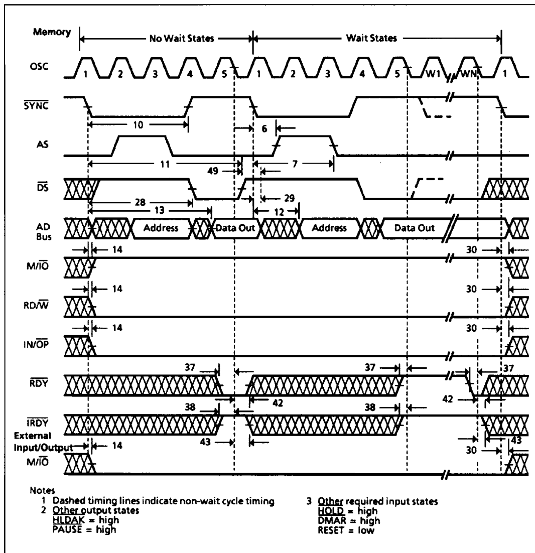
Figure 11: Write Transfer Timing
