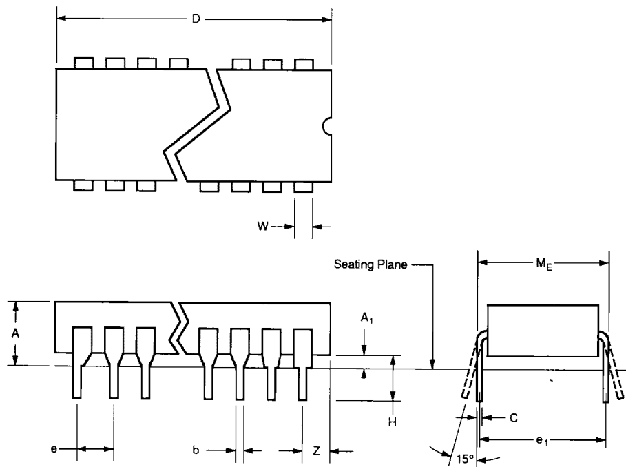
Figure 21a: 64-Lead Ceramic DIL - Package Style C
