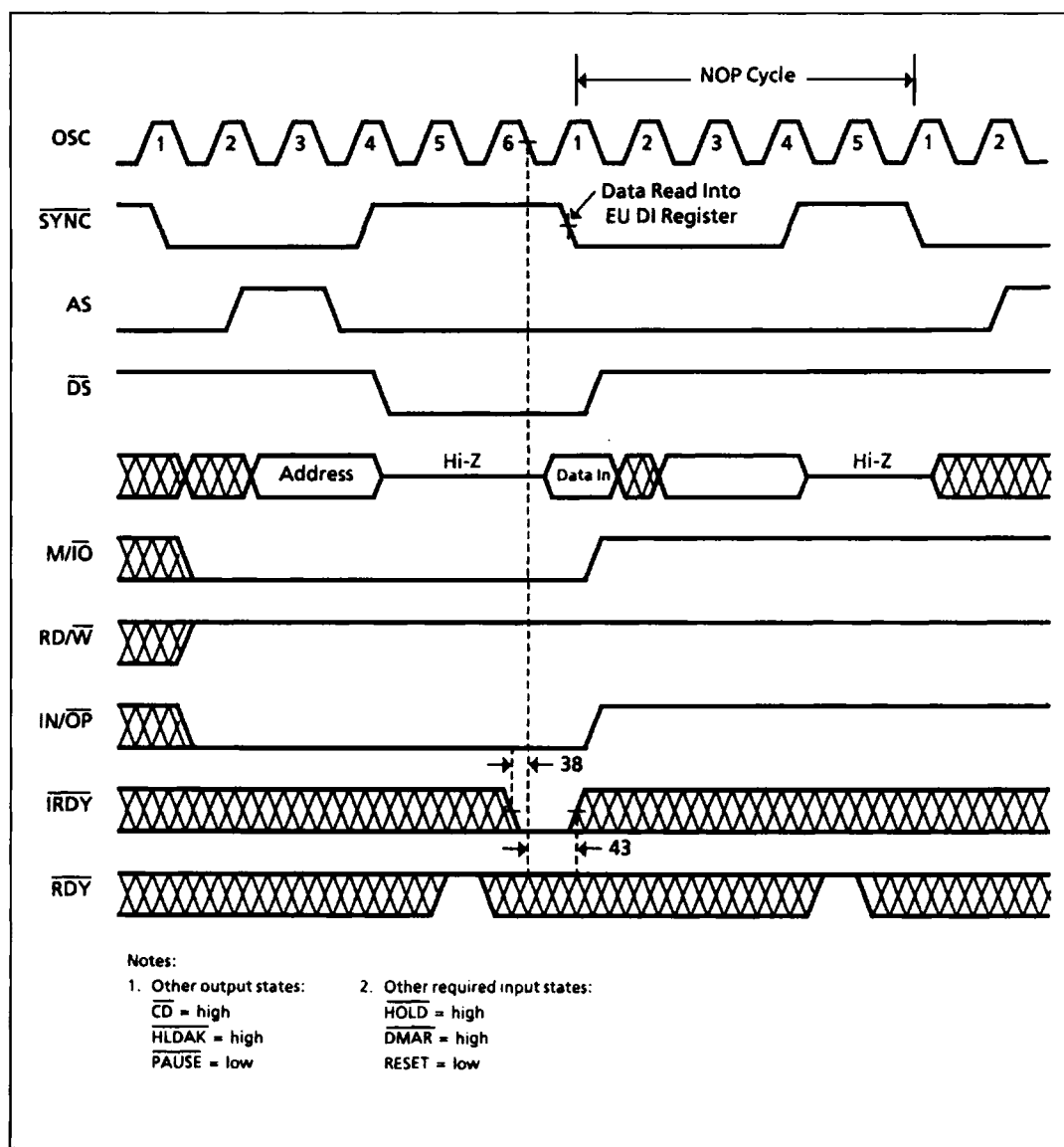
Figure 14: Internal I/O Timing - Read
