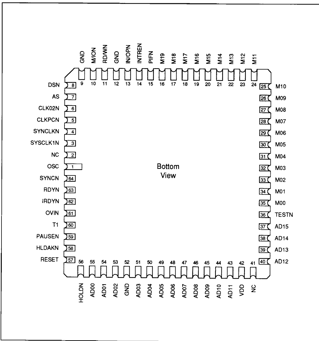
Figure 22b: Pin Assignments
