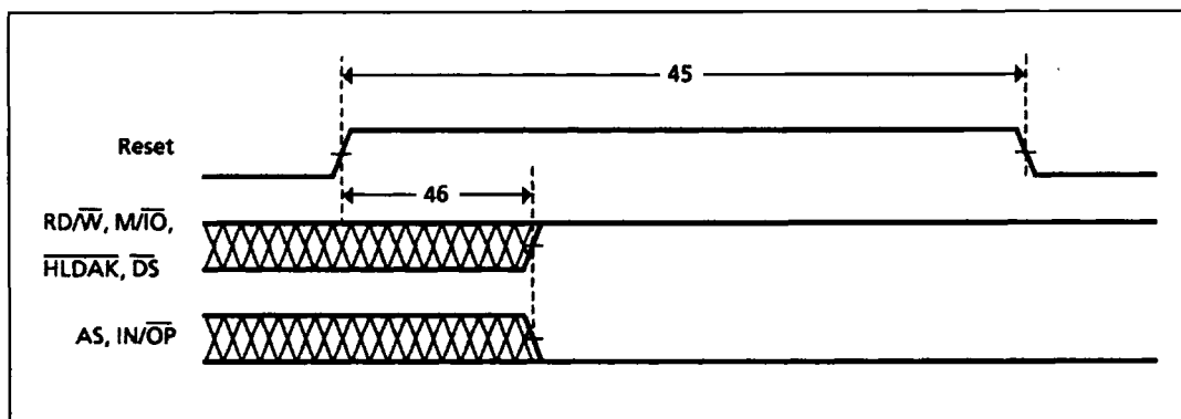
Figure 6: Reset Timing
