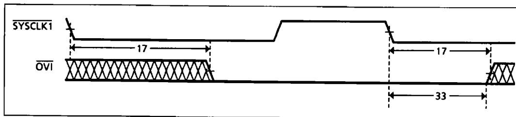
Figure 18: Fixed Point Overflow Timing
