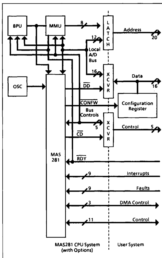
Figure 4: Typical MAS281/MA17504 System Interface
