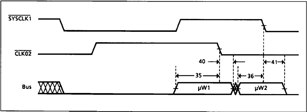
Figure 9: Microcode Bus Timing
