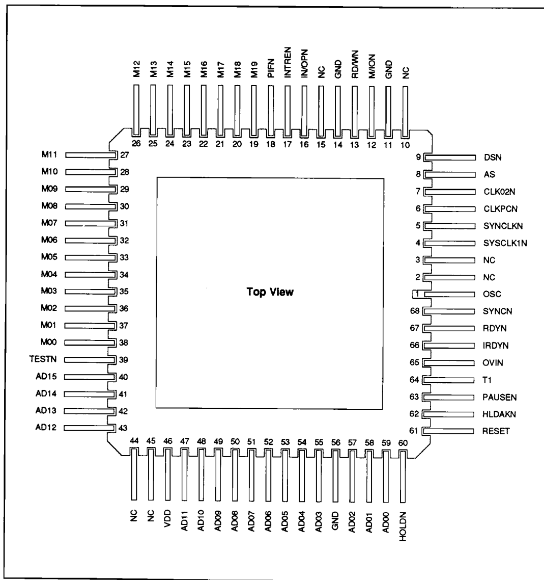
Figure 23b: Pin Assignments
