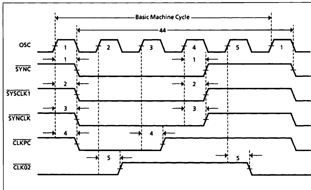
Figure 7: Basic Clock Timing
