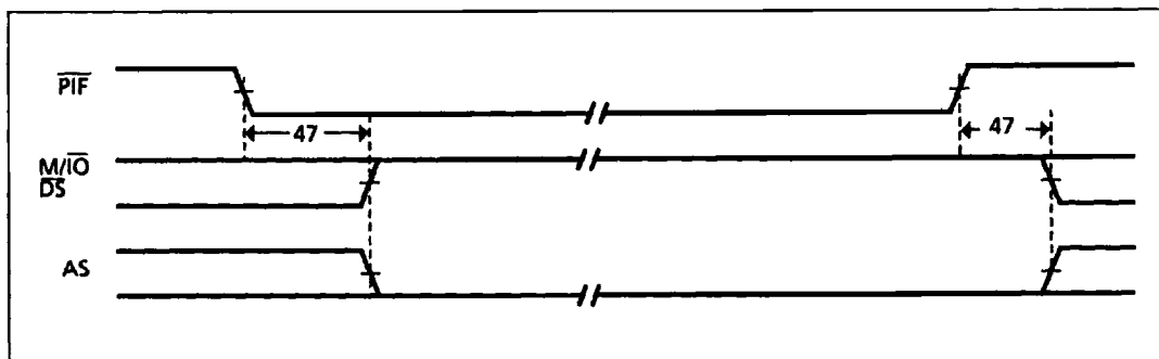
Figure 19: Instruction Abort Fault Timing
