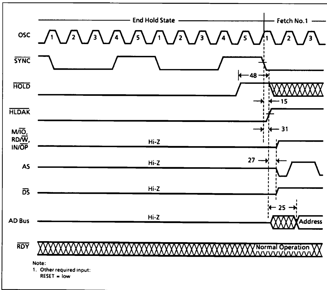
Figure 17: Hold State Termination Timing
