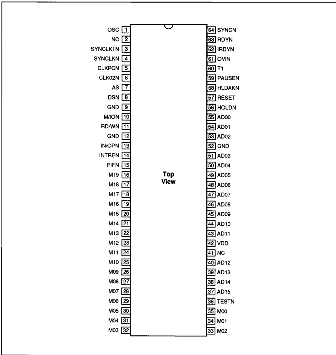
Figure 21b: Pin Assignments
