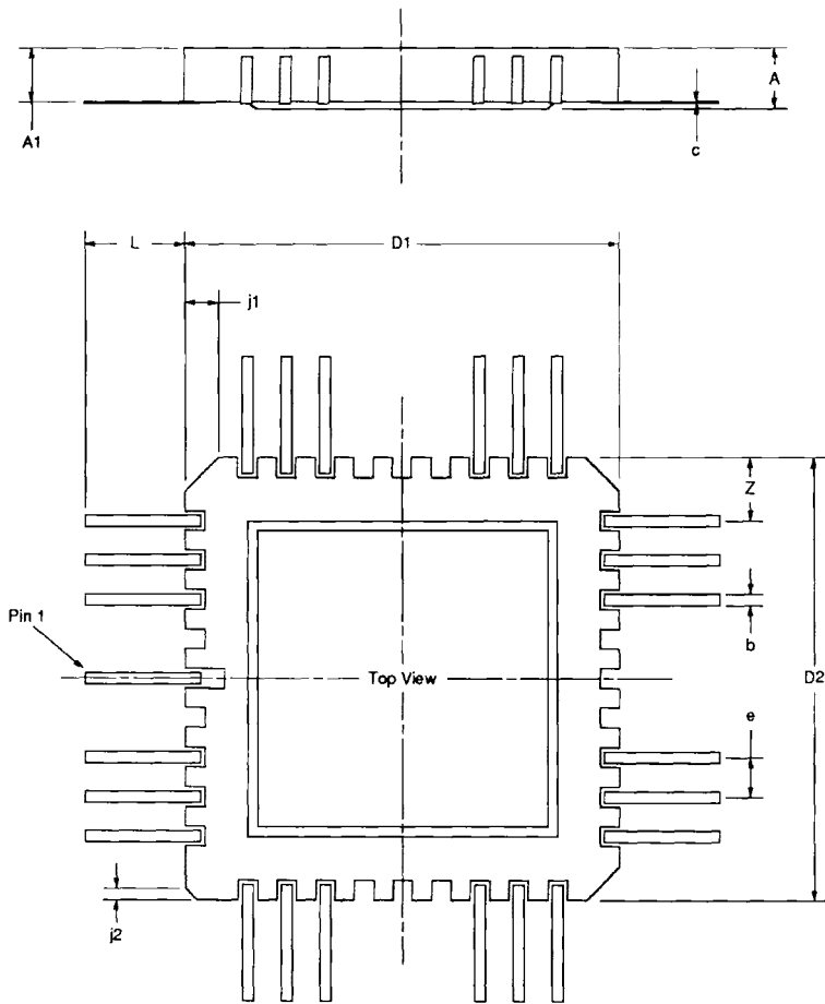
Figure 23a: 68-Lead Topbraze Flatpack - Package Style F
