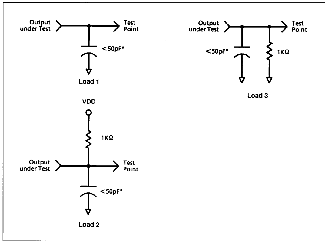
Figure 5: Test Loads
