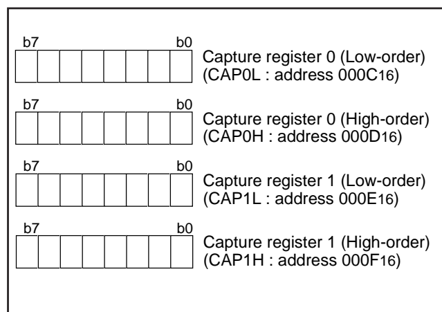
Fig. 42 Structure of capture software trigger register
