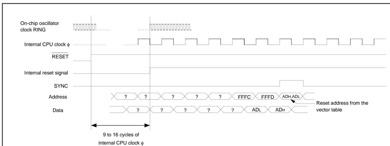
Fig. 68 Timing diagram at reset
