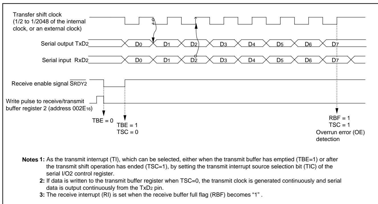
Fig. 57 Operation of clock synchronous serial I/O2 function
