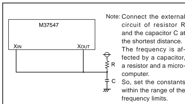
Fig. 72 External circuit of RC oscillation
