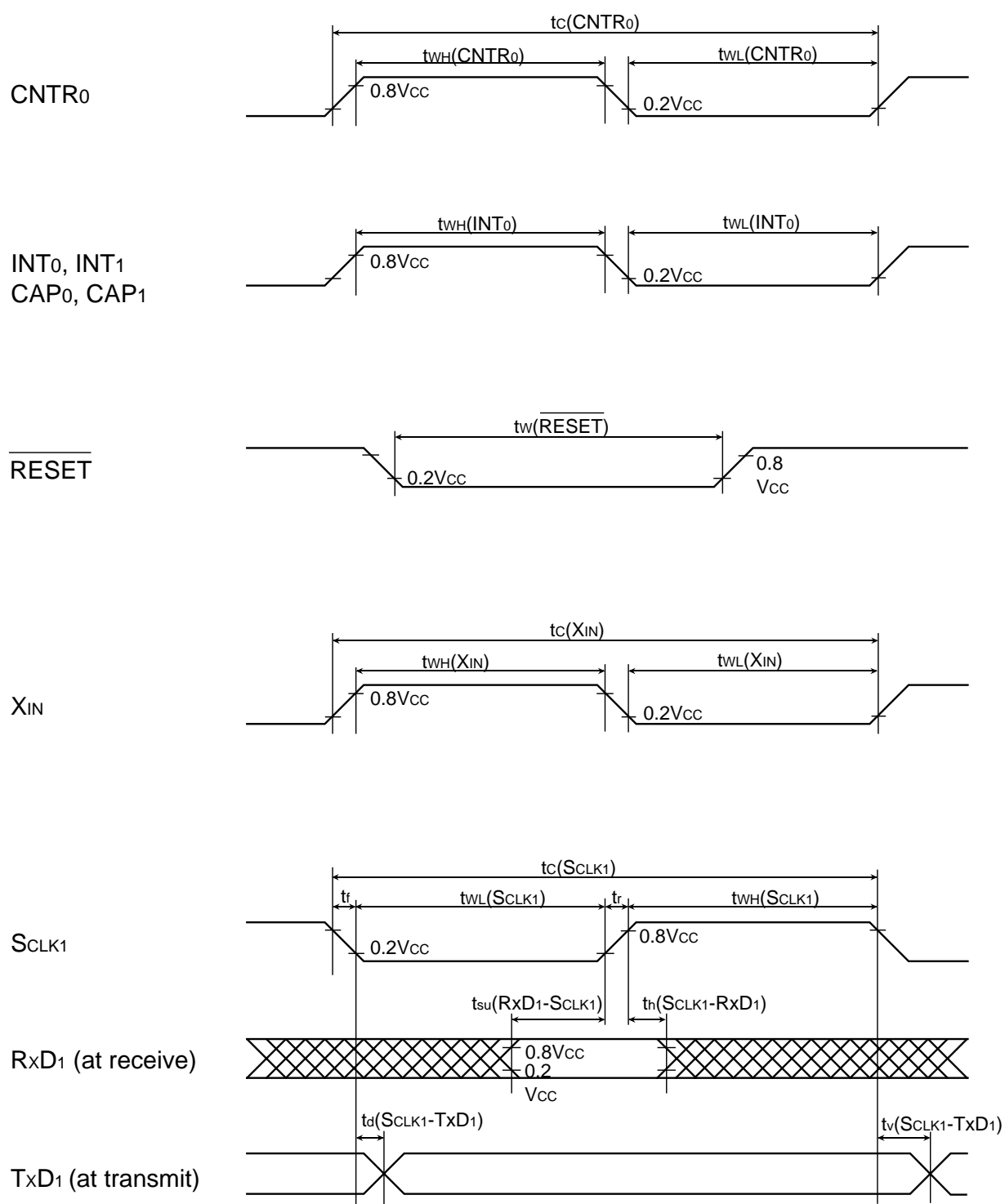
Fig. 101 Timing chart
