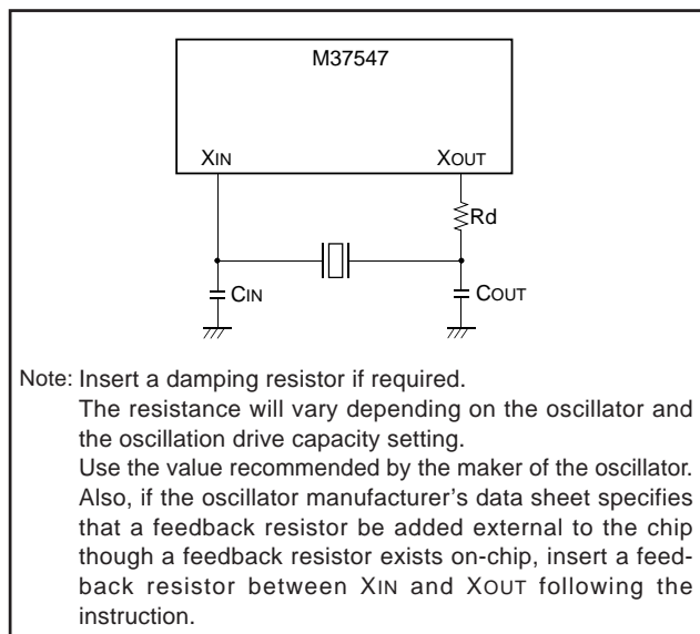
Fig. 71 External circuit of ceramic resonator
