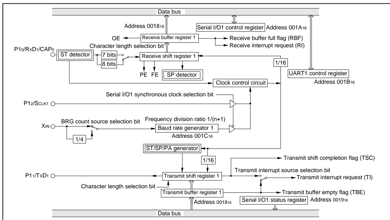
Fig. 50 Block diagram of UART serial I/O1
