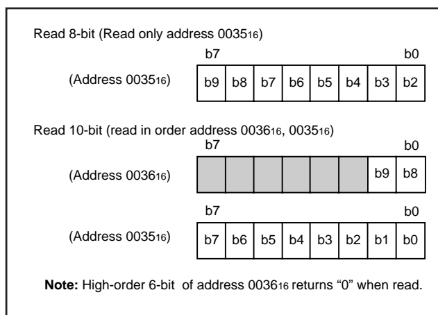
Fig. 62 Structure of A/D conversion register
