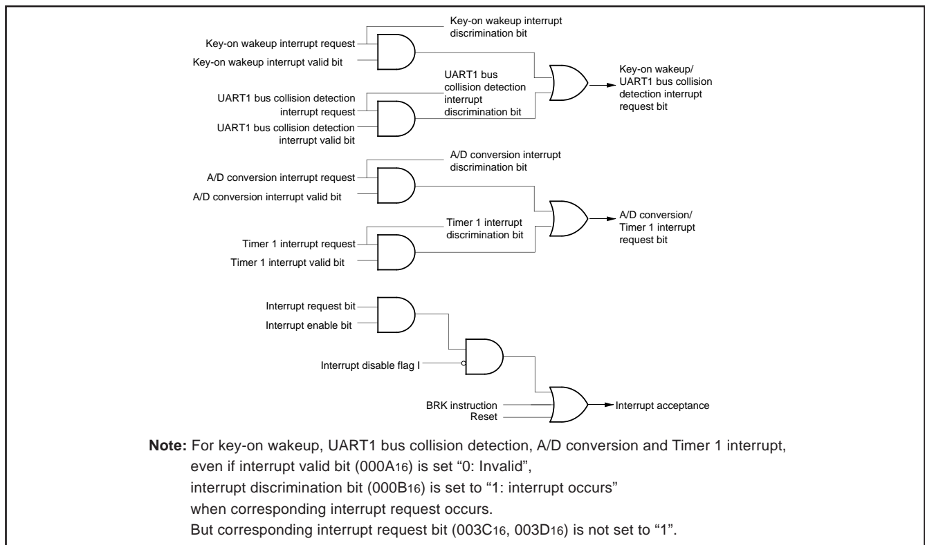
Fig. 16 Interrupt control
