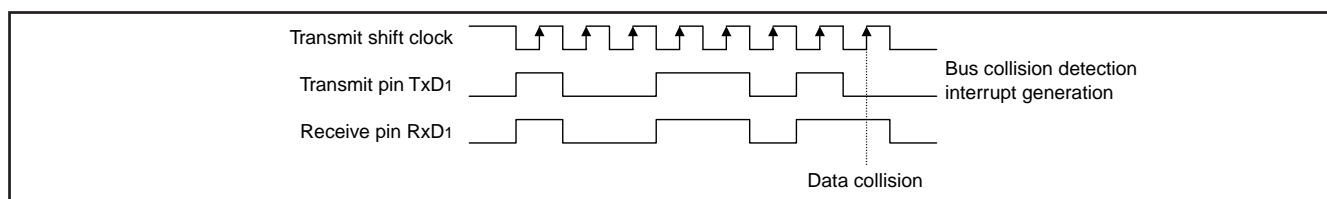
Fig. 55 Timing diagram of bus collision detection interrupt
