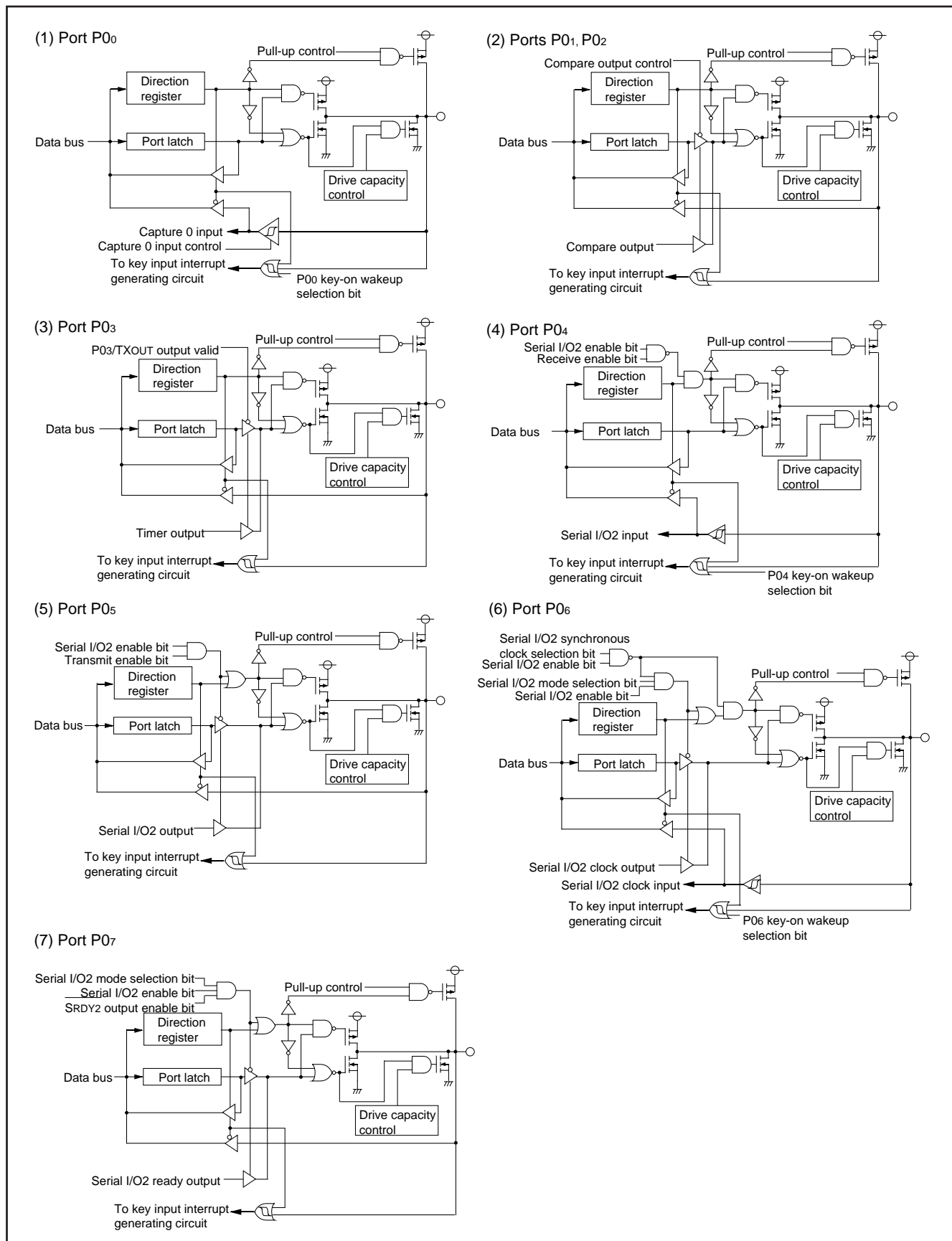
Fig. 13 Block diagram of ports (1)
