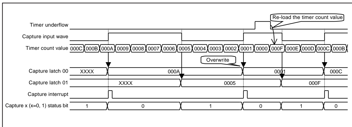
Fig. 46 Capture interrupt edge selection = “rising edge”
