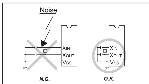
Fig. 90 Wiring for clock I/O pins
