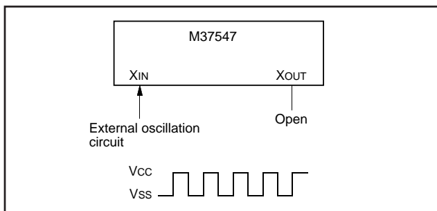
Fig. 73 External clock input circuit
