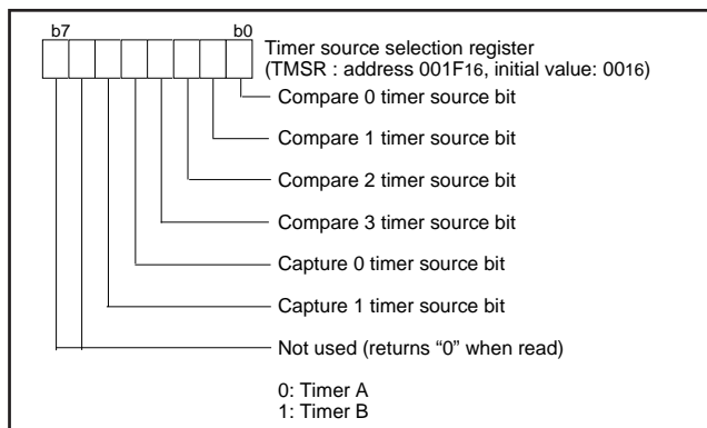
Fig. 31 Structure of timer source selection register
