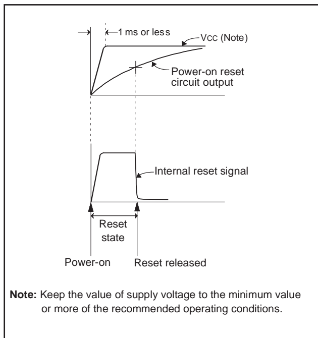
Fig. 66 Operation waveform diagram of power-on reset circuit
