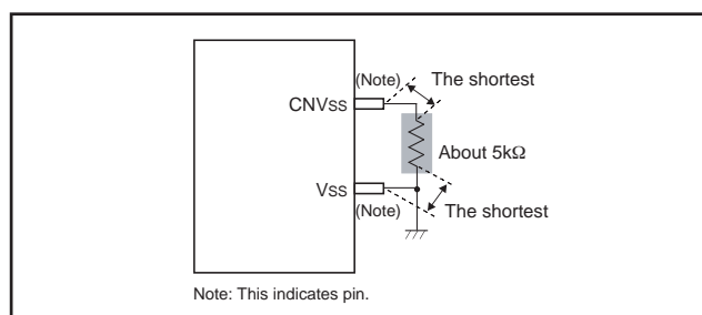
Fig. 91 Wiring for the CNVss pin of the QzPROM
