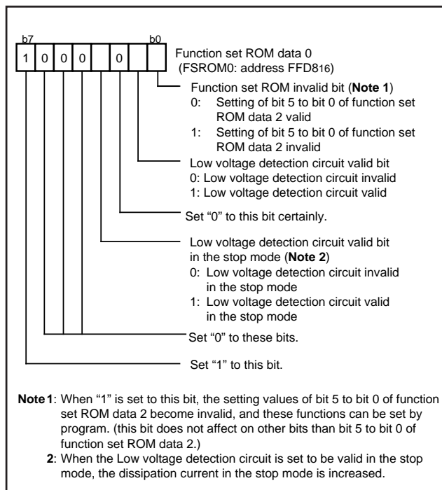
Fig. 82 Structure of Function set ROM data 0
