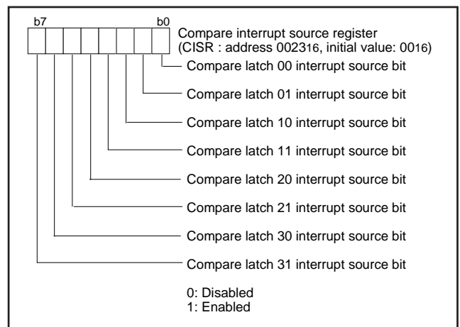
Fig. 34 Structure of compare interrupt source register
