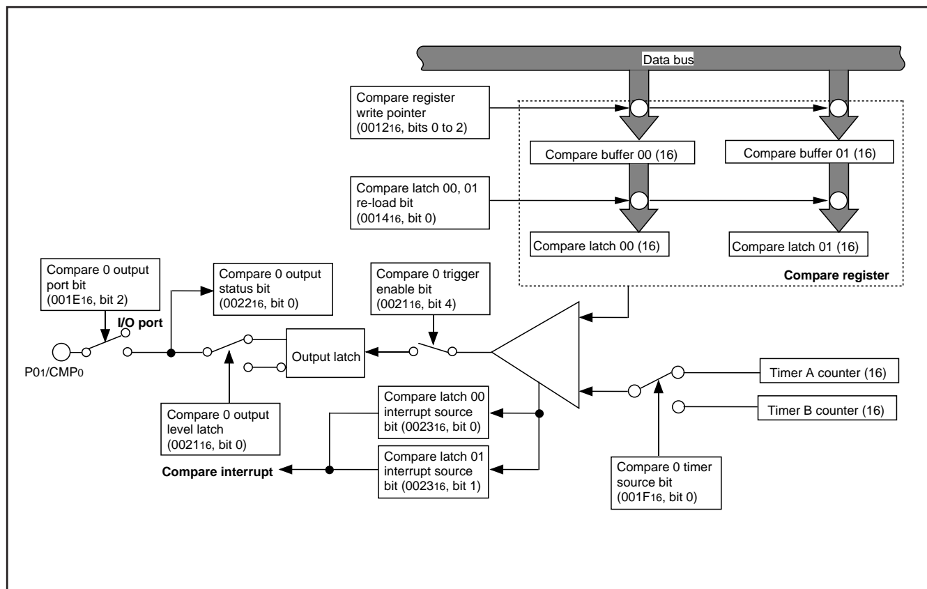
Fig. 36 Block diagram of compare channel 0
