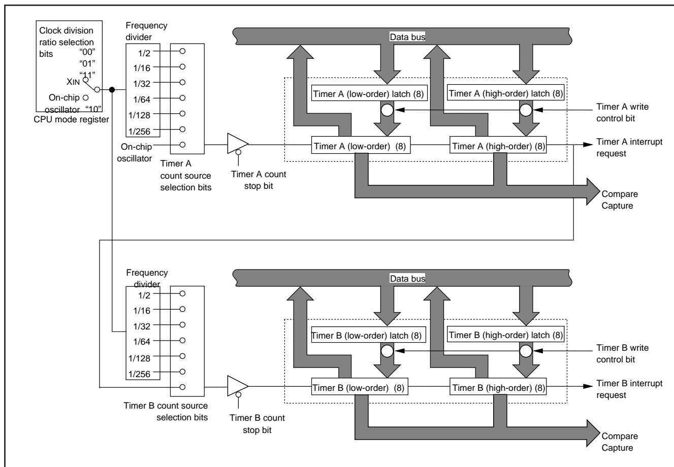
Fig. 27 Block diagram of timer A and timer B
