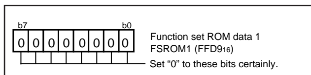
Fig. 83 Structure of Function set ROM data 1
