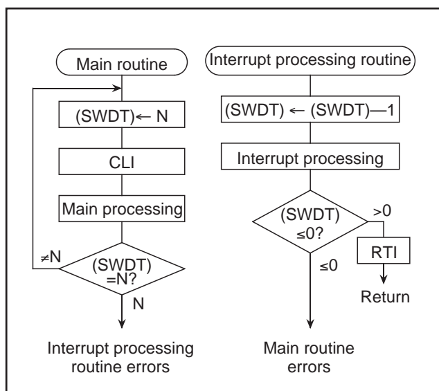
Fig. 97 Watchdog timer by software
