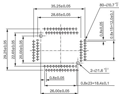
QFP IC234-0804-001 (80 Pins)
