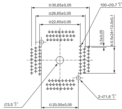
QFP IC234-1004-023 (100 Pins)
