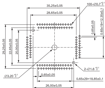
QFP IC234-1004-033 (100 Pins)
