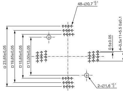
QFP IC234-0484-034 (48 Pins)
