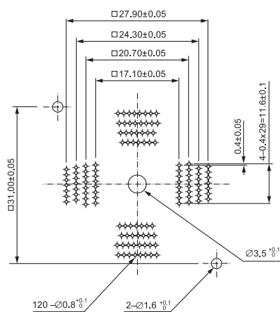
QFP IC234-1204-022 (120 Pins)
