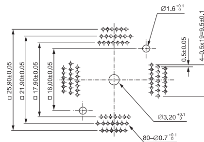
QFP IC34-0804-011 (80 Pins)
