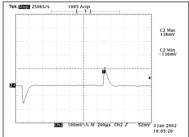
FIGURE 9: Output voltage response to step-change in load current. 50\% I_o to 75\% I_o , where di/dt = 1A/\mu s Load cap: 470\mu F , 30\text{ m}\Omega ESR tantalum capacitor and 1\mu F ceramic capacitor
