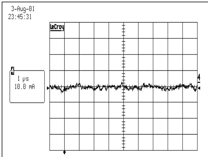
FIGURE 2: Input Reflected Ripple Current, set-up per figure 1; 10 \mu H source impedance. Nominal input voltage at full rated load.
