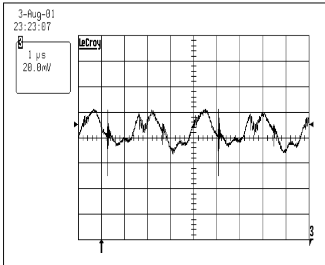
FIGURE 4: Output Voltage Ripple, set-up per figure 1; 1 \mu F ceramic capacitor and 10 \mu F tantalum capacitor. Nominal input voltage at full rated load
