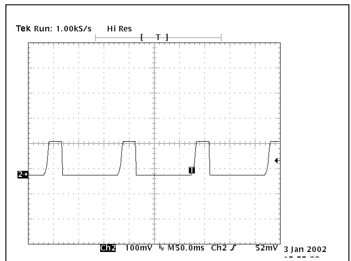
FIGURE 5: Load current as a function of time while attempting to enable into a short circuit, <10m \Omega .
