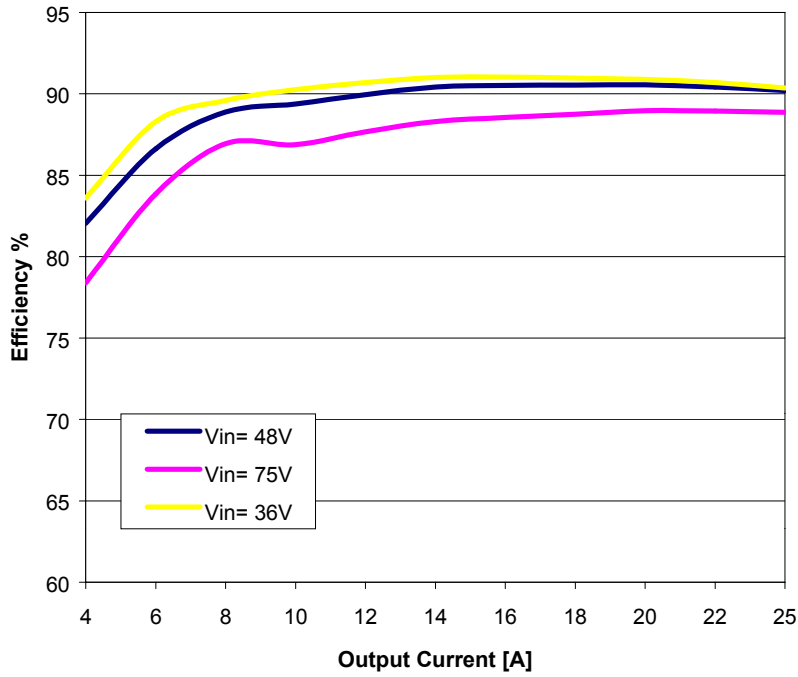
FIGURE 10: Efficiency vs. load current for different input voltages at 25°C
