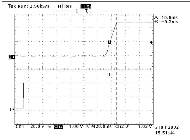
FIGURE 6: Turn-on transient at full rated load. Upper trace: output voltage. Lower trace: input voltage
