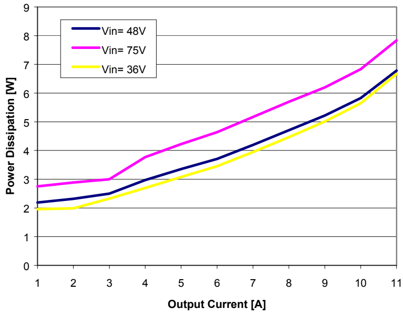
FIGURE 11: Power dissipation vs. load current for different input voltages at 25°C
