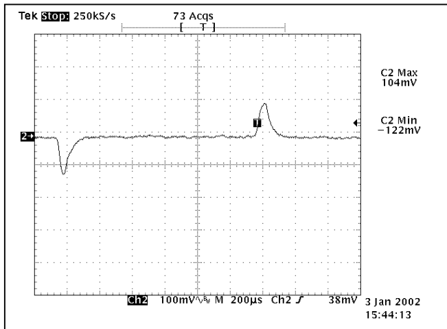
FIGURE 8: Output voltage response to dynamic change in load current: 75\% I_o to 50\% I_o , where di/dt = 0.1A/\mu s Load cap: 10\mu F , 100\text{ m}\Omega ESR tantalum capacitor and 1\mu F ceramic capacitor
