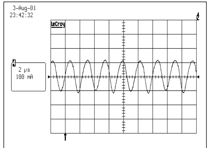
FIGURE 3: Input Terminal Ripple Current, set-up per figure 1; 10 \mu H source impedance and 47 \mu F electrolytic capacitor. Nominal input voltage at full rated load.
