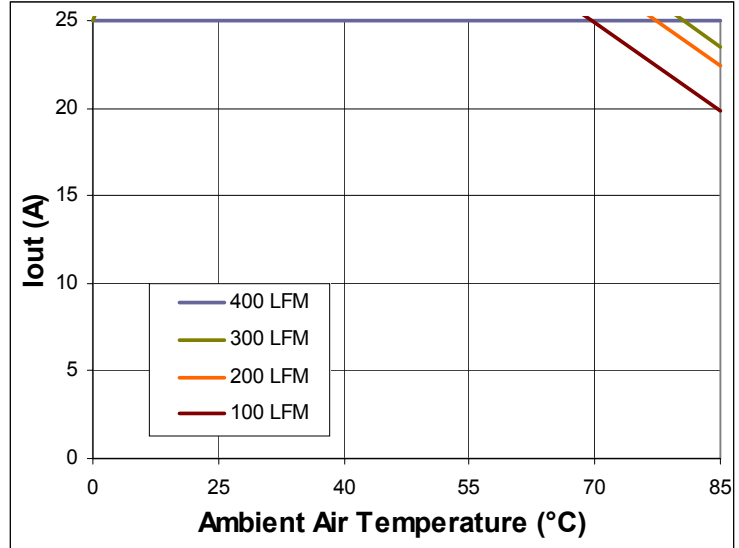
FIGURE 12: Maximum output current derating curves vs. ambient air temperature. Airflow rates of 100 LFM through 400 LFM with air flowing across the converter (Transversal) from pin 1 to pin 3 at nominal input voltage.
