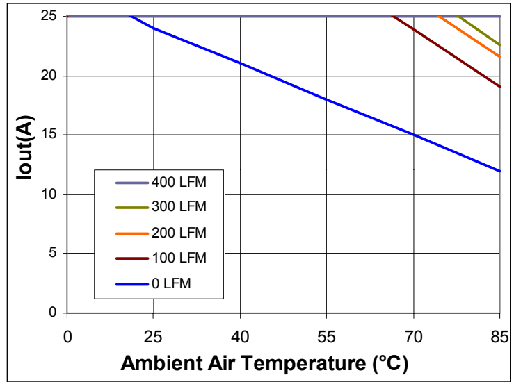
FIGURE 13: Maximum output current derating curves vs. ambient air temperature. Airflow rates of 0 LFM through 400 LFM with air flowing lengthwise from input to output at nominal input voltage.
