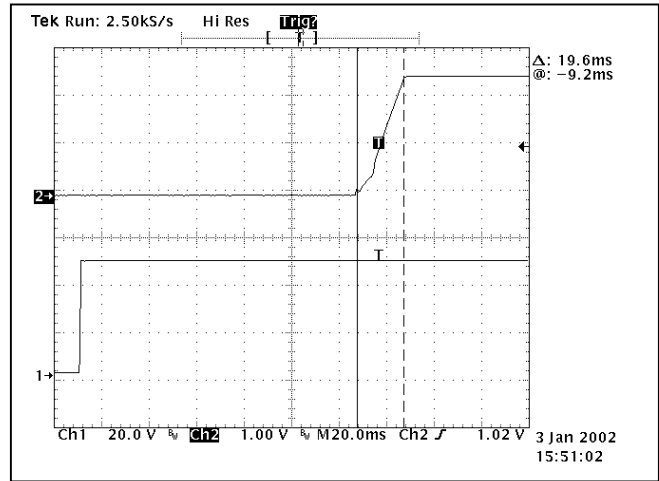
FIGURE 7: Turn-on transient at zero load. Upper trace: output voltage Lower trace: input voltage
