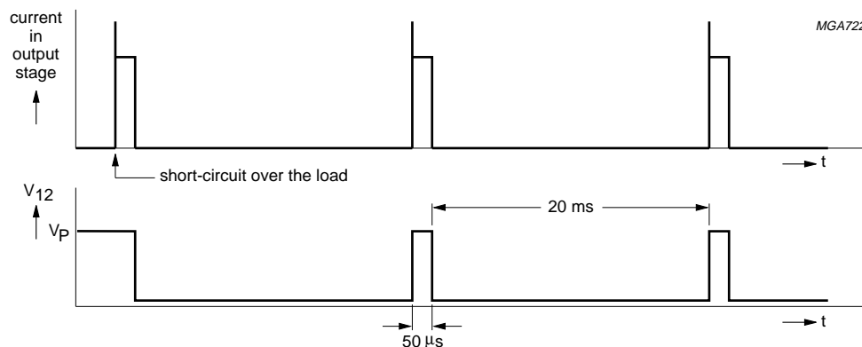
Fig.4 Short-circuit waveform.
