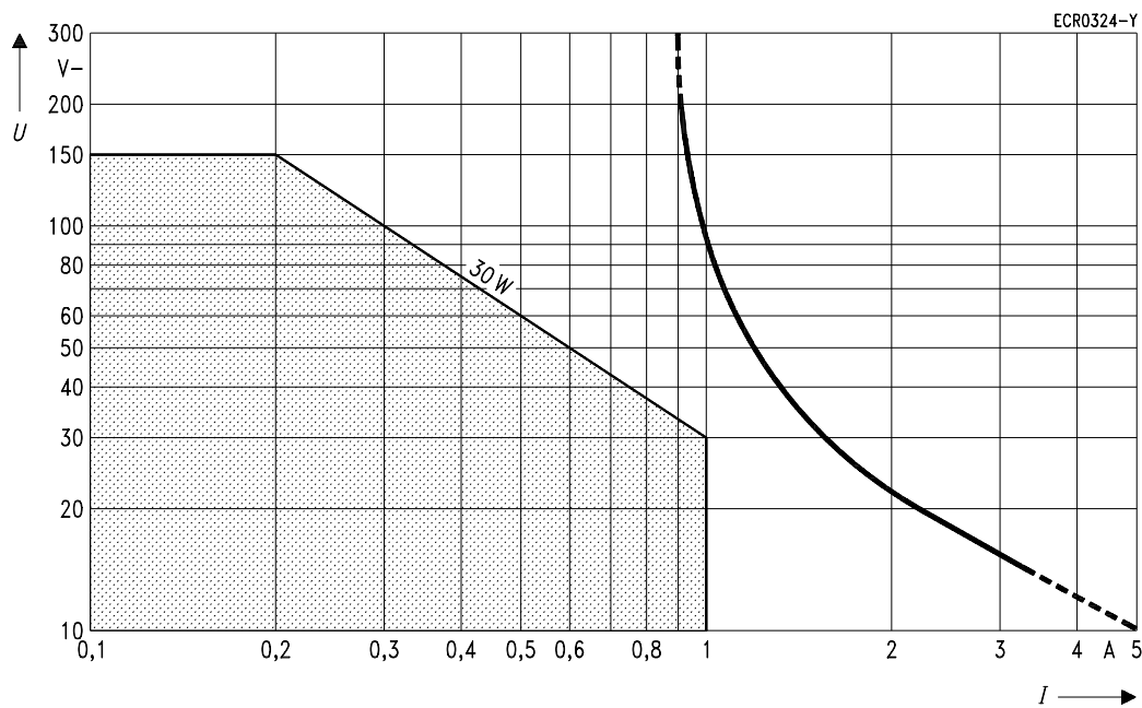
Load limit curve
