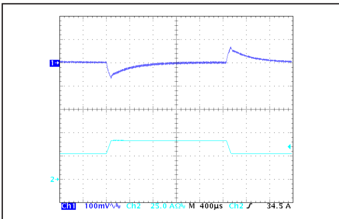
Figure 5: Output voltage response to step-change in load current (66%-100%-66% of Iout(max); dl/dt = 0.1A/μs). Load cap: 15μF tantalum cap and 1μF ceramic cap. Ch 1: Vout, Ch 2: Iout.
