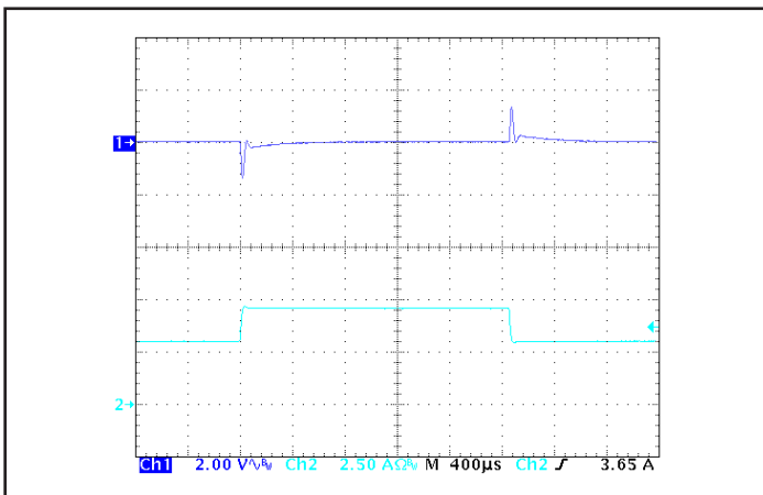
Figure 5: Output voltage response to step-change in load current (66%-100%-66% of Iout(max)); dl/dt = 0.1A/μs). Load cap: 1μF ceramic cap. Ch 1: Vout, Ch 2: Iout.
