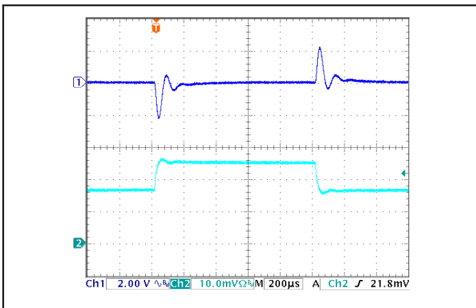
Figure 5: Output voltage response to step-change in load current (66%-100%-66% of Iout(max); dl/dt = 0.1A/μs). Load cap: 1μF ceramic cap. Ch 1: Vout, Ch 2: Iout (1 A/div).
