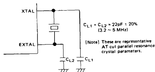
Figure 12 Crystal Interface
