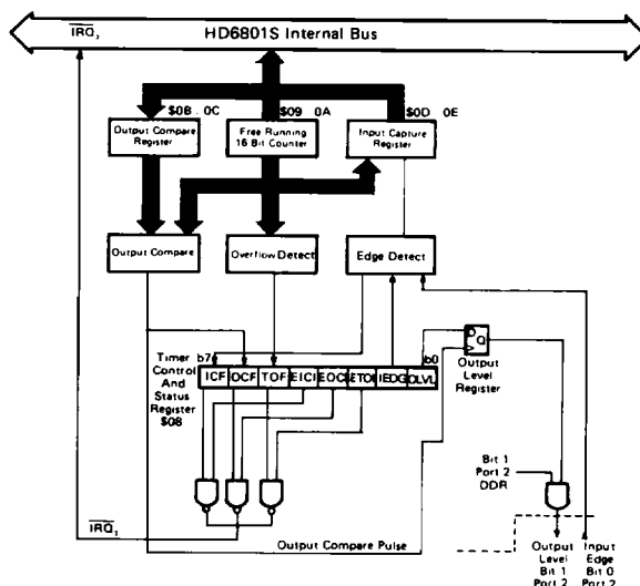
Figure 21 Block Diagram of Programmable Timer
