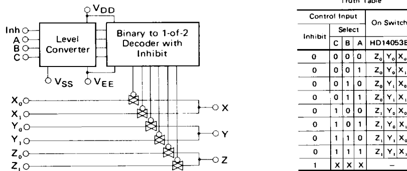
Figure 15 HD14053B Multiplexers/Demultiplexers
