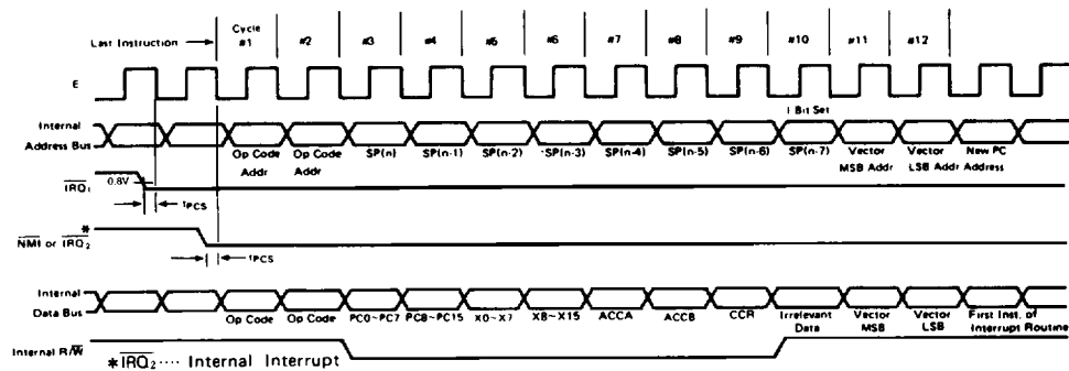
Figure 10 Interrupt Sequence
