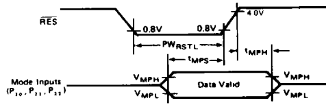
Figure 8 Mode Programming Timing
