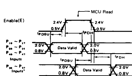
Figure 3 Data Set-up and Hold Times (MCU Read)
