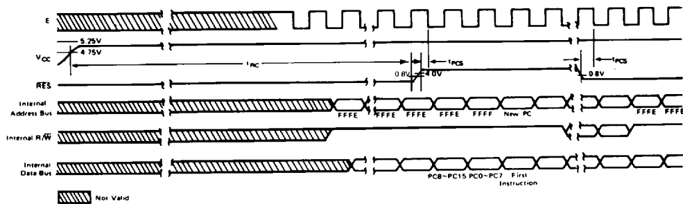
Figure 11 Reset Timing
