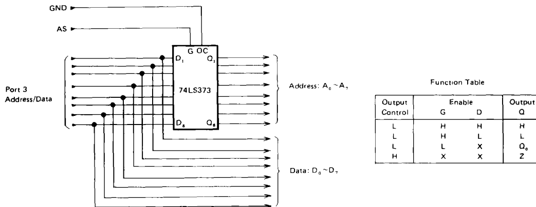
Figure 19 Latch Connection
