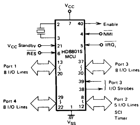
Figure 16 HD6801S MCU Single-Chip Mode
