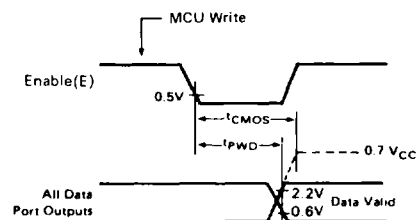
Figure 4 Port Data Delay Timing (MCU Write)
