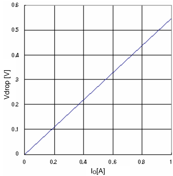
Fig.21 Minimum dropout Voltage 2 (Vcc=4.5V, Ta=25°C)
