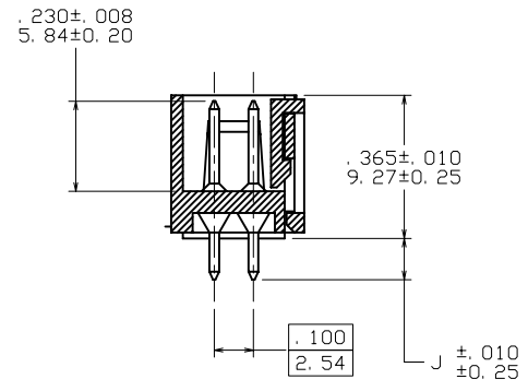
SECTION Z-Z
