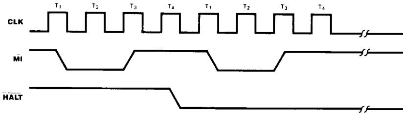
Figure 13. Power-Down Acknowledge
