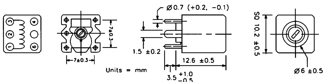
Style KM7 – Shielded with carbonyl E core and plastic sleeve
