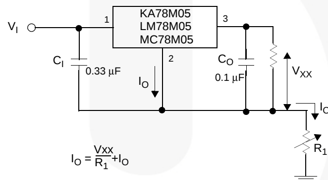
Figure 3. Constant-Current Regulator
