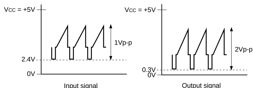
Fig. 10. CVBS/Y Waveforms
