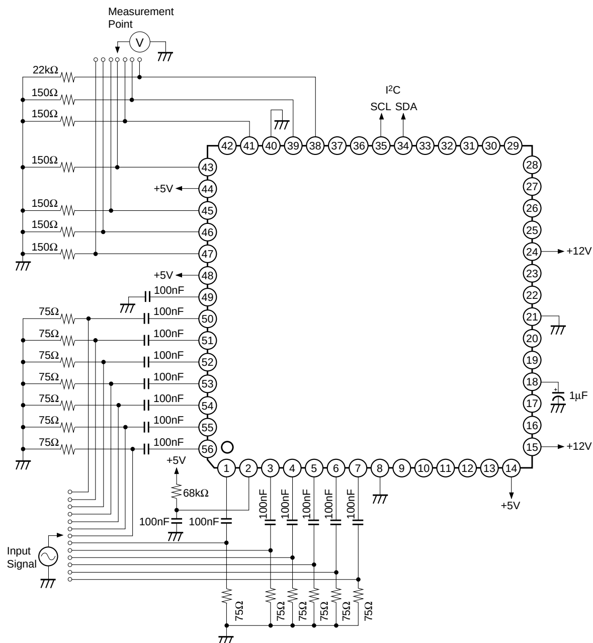
Fig. 2. Video System
