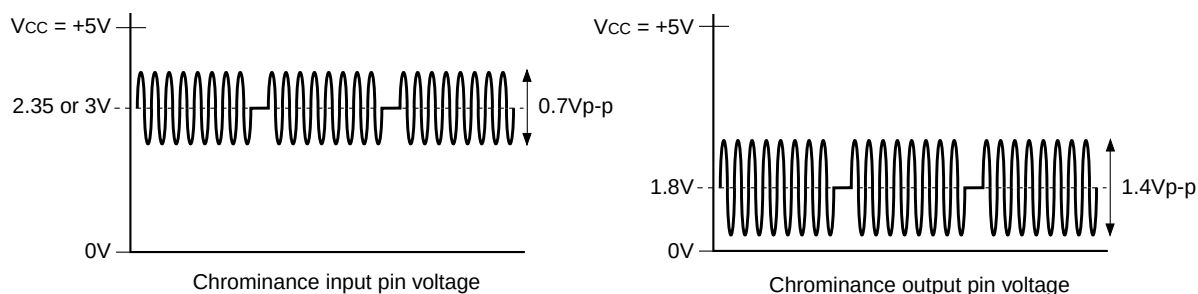
Fig. 13. Chrominance Waveforms
