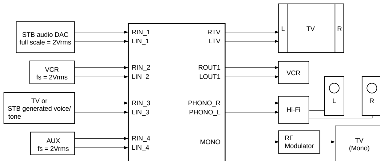
Fig. 23. Audio Application
