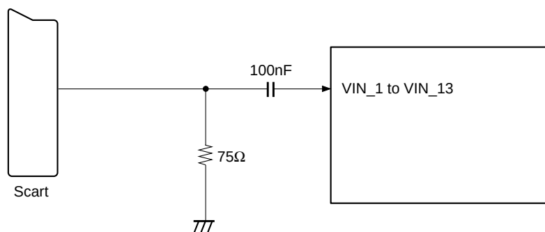
Fig. 15. Video Input Interface
