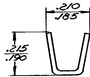
SECT. B-B
