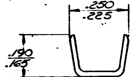
SECT. A-A
