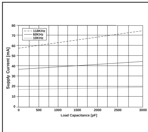
Figure 6. Supply Current VS. Load Capacitance when Transmitting Data for the SP3243
