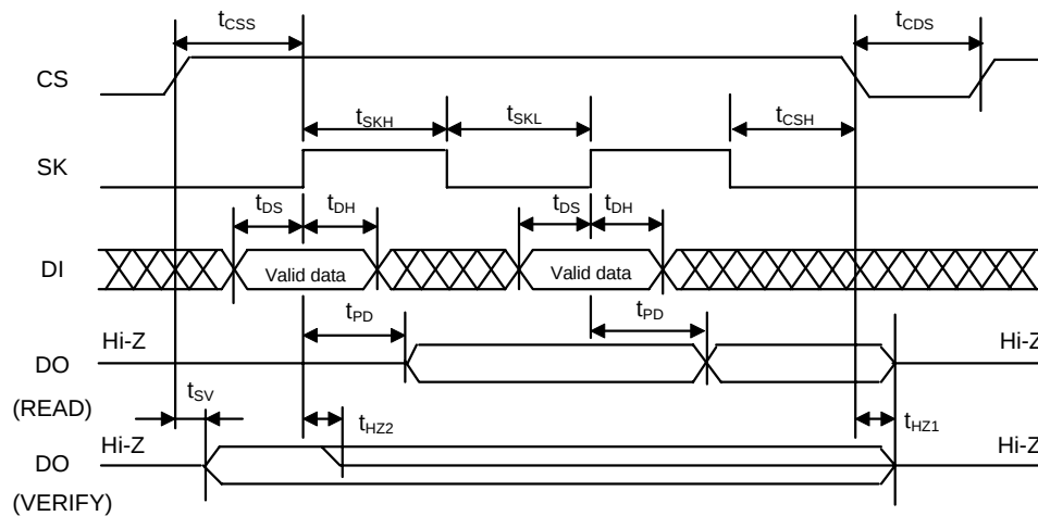
Figure 3 Read Timing
