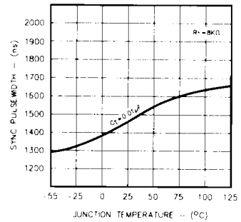
FIGURE 15. SYNC PULSEWIDTH VS. TEMPERATURE
