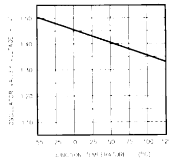
FIGURE 5. OSCILLATOR VALLEY VOLTAGE VS. TEMPERATURE
