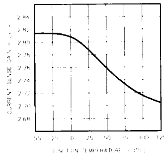
FIGURE 4. CURRENT SENSE GAIN VS. TEMPERATURE
