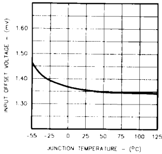
FIGURE 10. ERROR AMPLIFIER INPUT OFFSET VOLTAGE VS. TEMPERATURE
