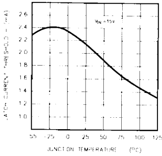
FIGURE 7. MINIMUM SCR LATCH CURRENT
