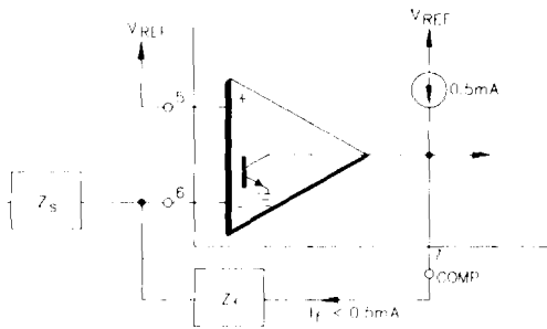
FIGURE 21 - ERROR AMP OUTPUT CONFIGURATION (Error amplifier can source up to 0.5mA)
