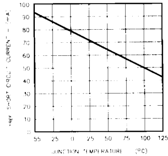
FIGURE 2. V_{REF} SHORT CIRCUIT CURRENT VS. TEMPERATURE
